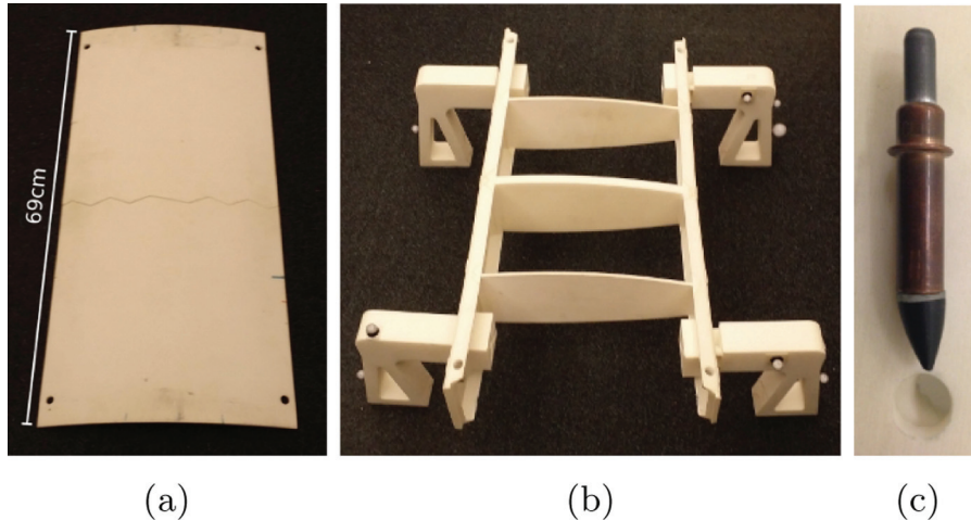
Fig. 2. Assembly parts used in our experiments. (a) Wing panel. (b) Wing box. (c) A fastener and hole (misaligned) as used in this task. The fastener is an adapted cleco. The holes were drilled to permit a cleco to fit up to the flange with a tolerance of 1.5 mm.
