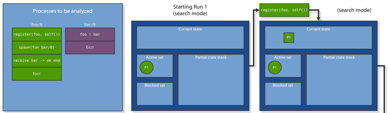
Figure 4.4: Testing the example of Listing 4.2 using depth-first search with blocking avoidance (cont'd on the next page)
