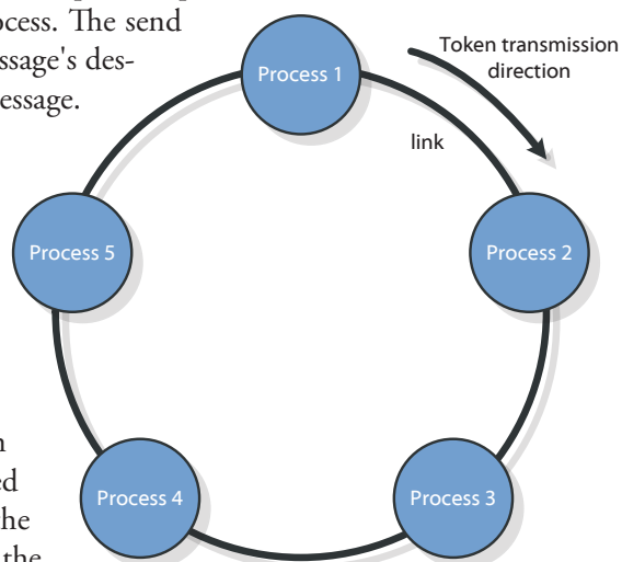
Figure 2.1: The ring of linked processes created by the program of Listing 2.2.
