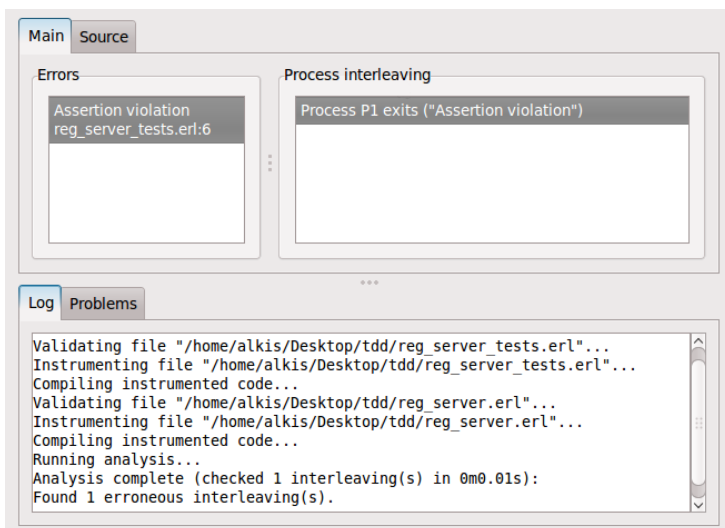
Figure 6.2: Information about an erroneous interleaving
