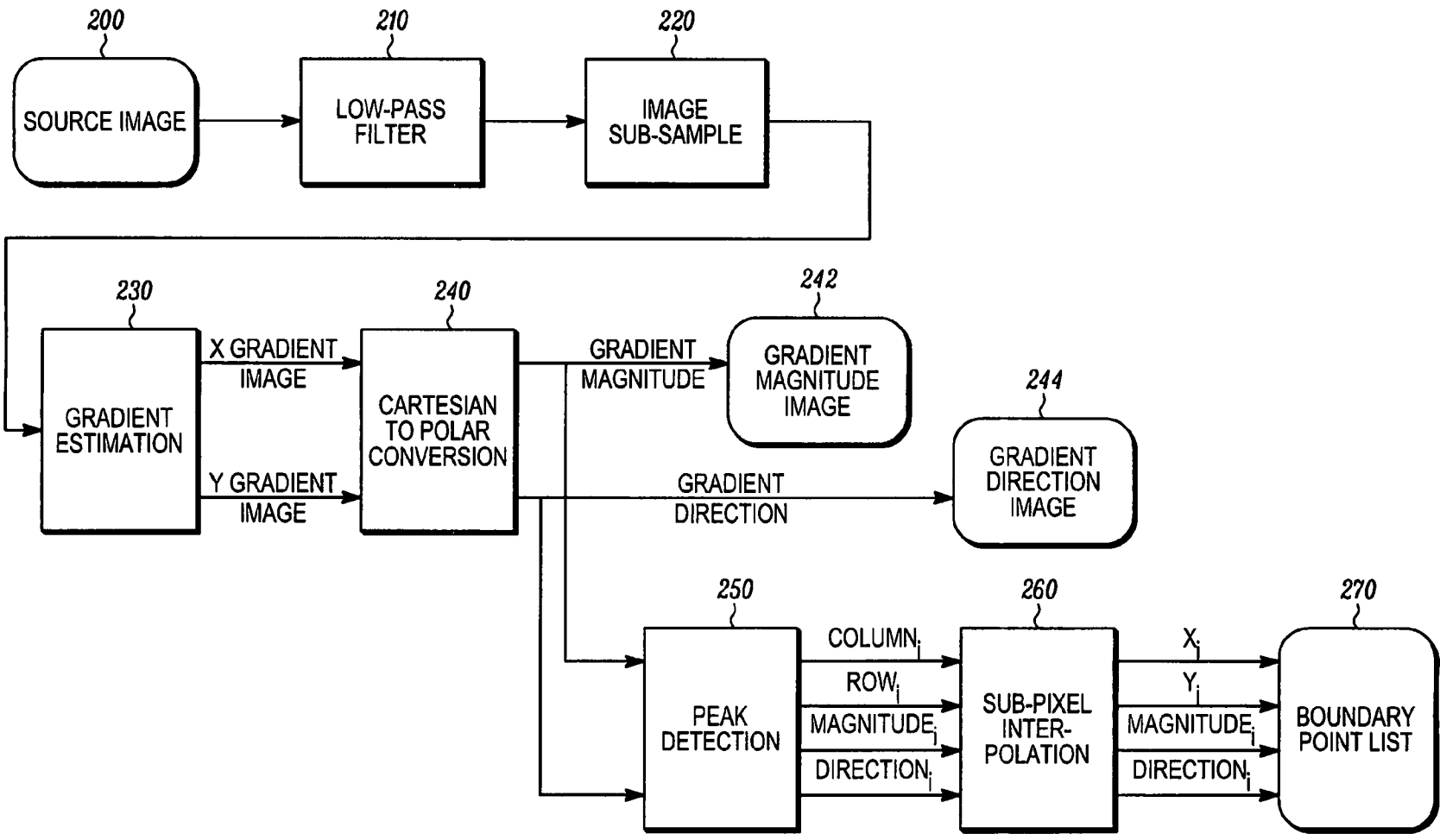
GRANULARITY CONTROL, GRADIENT, AND BOUNDARY DETECTION
