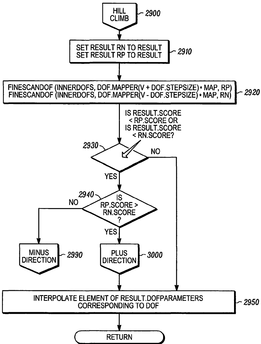
FINE SCAN HILL CLIMBING
