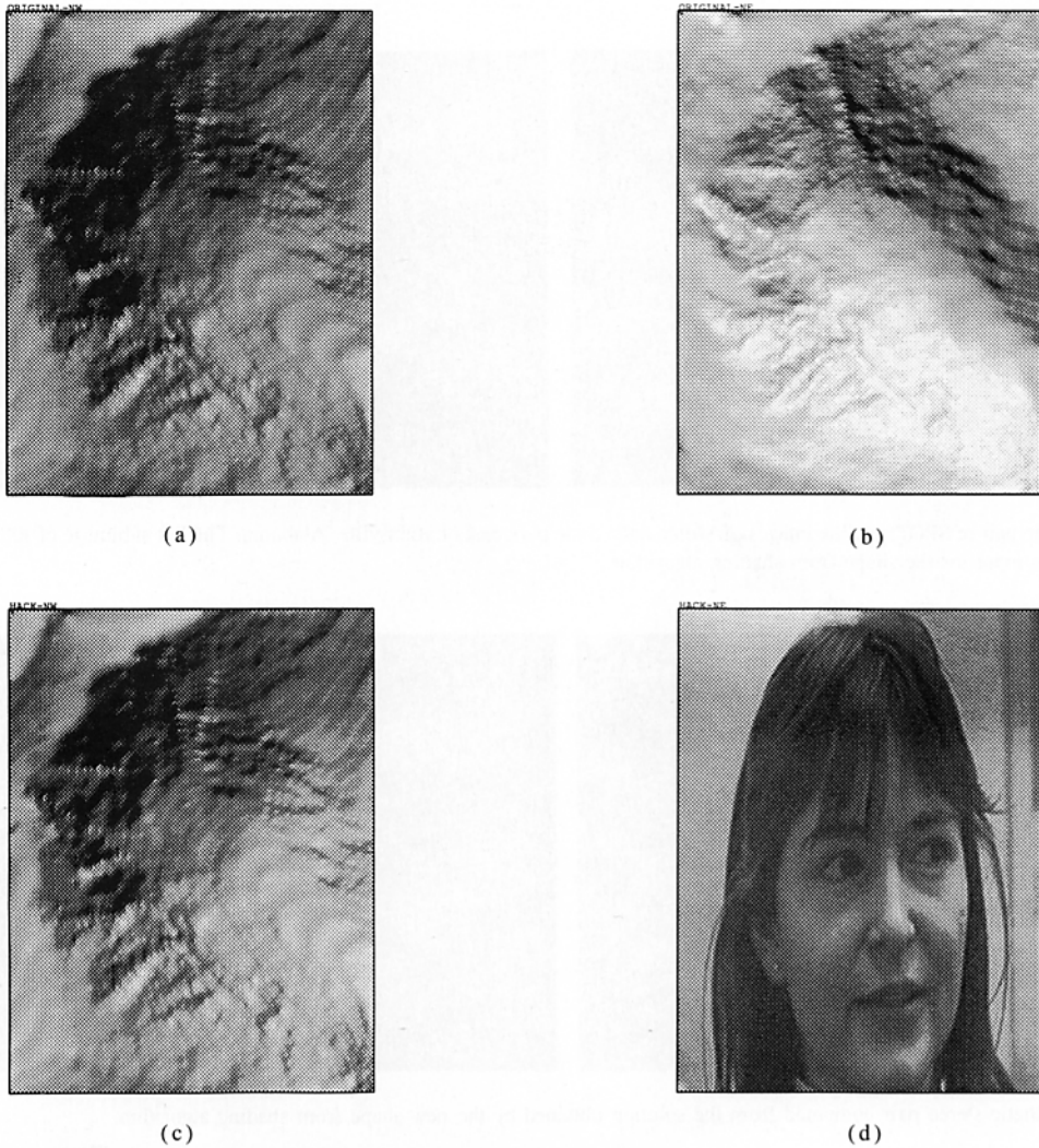
Fig. 12. New one-step shape-from-shading algorithm, See text!
