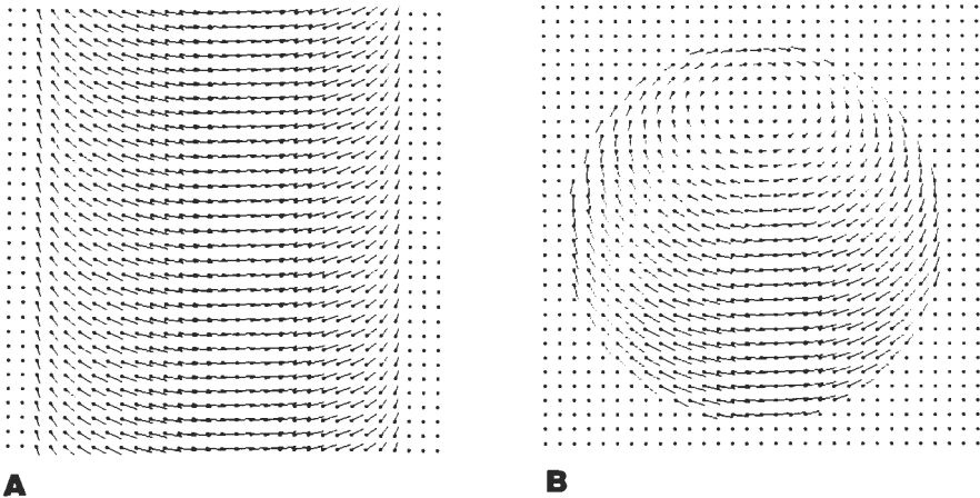
FIG. 11. Exact flow patterns for the cylinder and the sphere.
