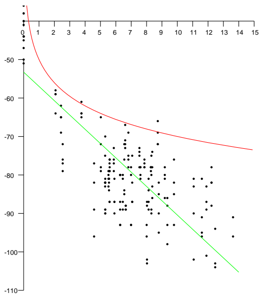
Fig. 1. Scattergram of Signal Strength (RSS) versus distance in typical three-level wooden building. Horizontal axis: distance between smartphone and APs (in meters). Vertical axis: Signal Strength (in dBm). Red curve: expected inverse square law dependence ( -50 - 20 \log(R) dBm). Green line: linear fit ( -53 - 3.7R dBm). Because of the large scatter, it should be clear that RSS is not very useful for estimating distance.
