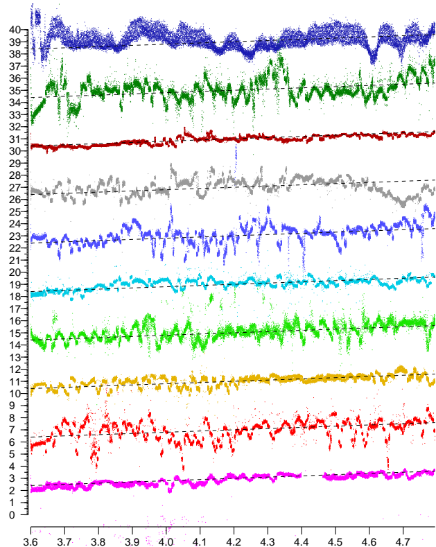
Fig. 3. Sample measurements using ten responders in a range of positions (Top plot is for an access point operating in the 2.4 GHz band, the rest are in the 5 GHz band). Horizontal axis: actual position in meters. Vertical axis: reported distances in meters. (Note that the average slope of the plots is not equal to one, because the scales on the vertical axis and horizontal axes are different). (Individual plots are offset vertically to avoid overlap).
