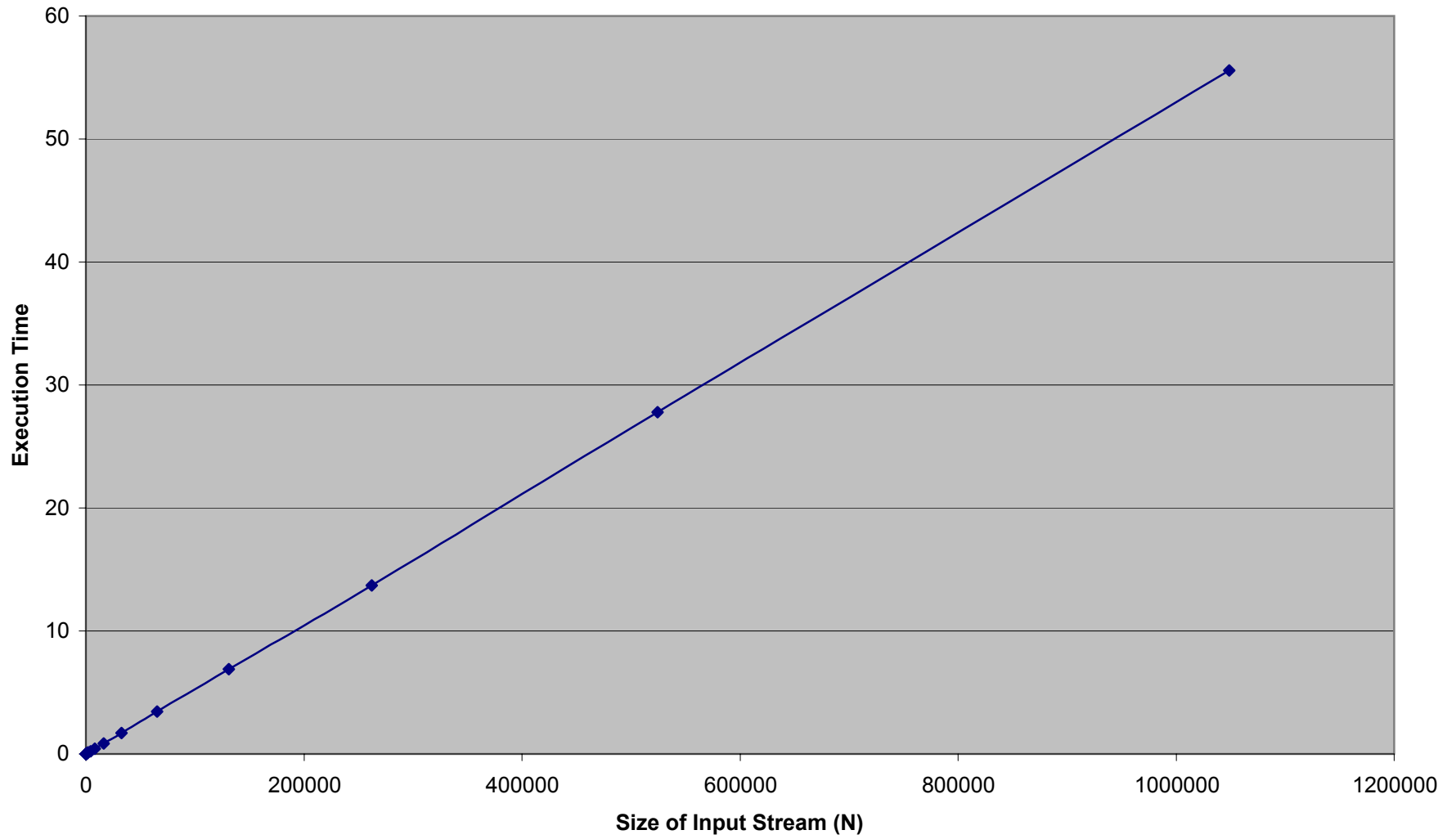
O(N) timed_test_1c
