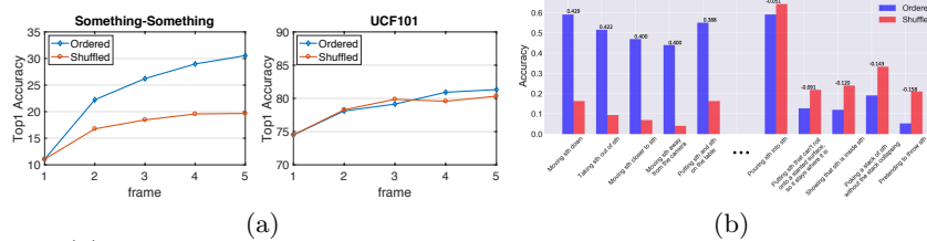
Fig. 6: (a) Accuracy obtained using ordered frames and shuffled frames, on Something-Something and UCF101 dataset respectively. On Something-Something, the temporal order is critical for recognizing the activity. But recognizing activities in UCF101 does not necessarily require temporal relational reasoning. (b) The top 5 action categories that exhibited the largest gain and the least gain (negative) respectively between ordered and shuffled frames as inputs. Actions with directional motion appear to suffer most from shuffled inputs.
