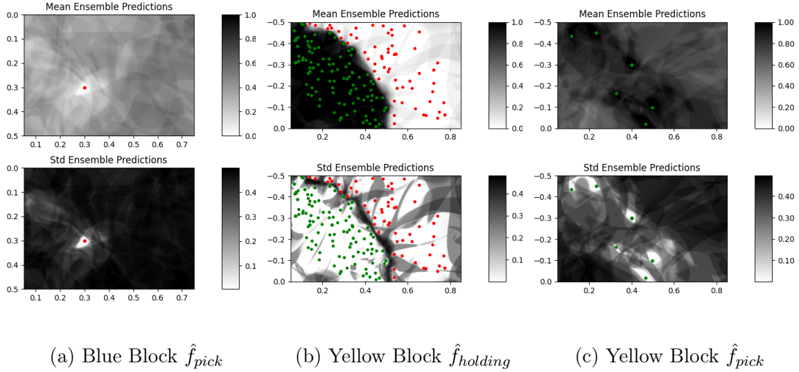
Figure 7-10: Learned action feasibility model predictions for Sequential Actions. These plots show the ensemble predictions of the AFMs learned from a single run of the Sequential Actions strategy. The grayscale color indicates the model’s prediction for the given (x, y) input (see Section 7.3.2 for the model inputs). In the top mean prediction plots, a value of 1.0 indicates feasible action parameters, and 0.0 indicates infeasible action parameters. In the bottom standard deviation plots the value indicates the standard deviation of the ensemble’s prediction for a given AFM input. The plotted points are the action parameters which were executed by the learning strategy and were found to be either feasible (green) or infeasible (red). Only the actions that were used to train the AFMs are visualized. Many other actions (such as MoveFree) were executed, but not used to learn an AFM and thus are not visualized here. For the blue block, the robot attempts to pick it from its initial position, but finds that that action is infeasible. It never explores plans to first push the blue block out of the tunnel, therefore no other pick actions are ever successful. For the yellow block the robot is able to successfully pick it up from its initial position. It is then able to learn that some MoveHolding actions are feasible while others are not. The Sequential Actions strategy leads the robot to execute a plan which involve picking, placing, then picking up the yellow block again. This is shown by the Pick attempts which do not correspond to the yellow block’s initial position. No MoveContact actions are ever attempted due to the difficulty of randomly sampling a successful tool use plan when generating P_{act} .
