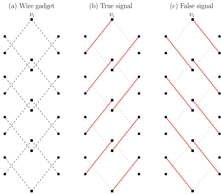
Figure 3: Wire gadget.
