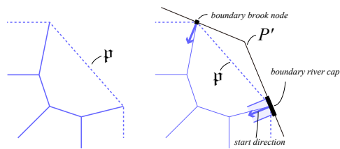
■ Figure 8 Left: Tutte embedding with outside face p . Right: Construction of start ray and convex polygon P' .
