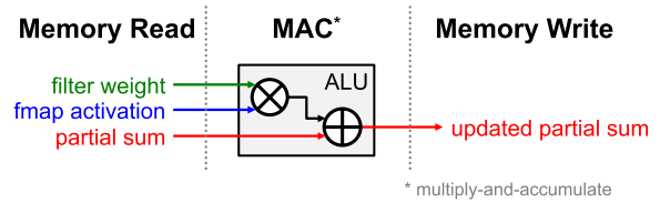
Fig. 21. Read and write access per MAC.
