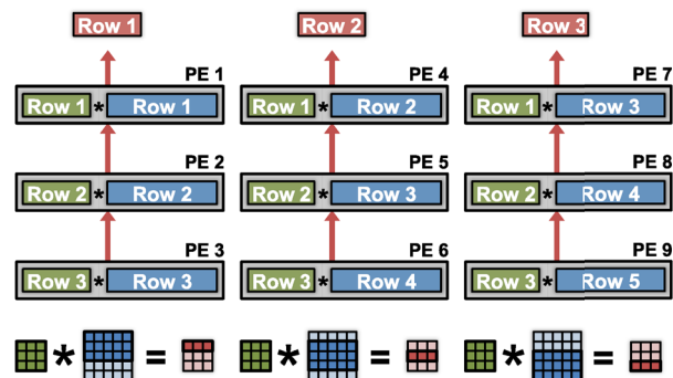
Fig. 28. Two-dimensional convolutional reuse within spatial array for row stationary dataflow [82].
