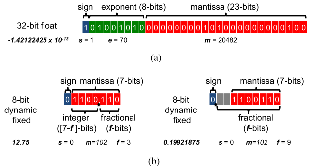
Fig. 38. Various methods of number representations. (a) 32-bit floating point example. (b) 8-bit dynamic fixed point examples.
