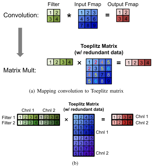
Fig. 19. Mapping to matrix multiplication for convolutional layers. (a) Mapping convolution to Toeplitz matrix. (b) Extend Toeplitz matrix to multiple channels and filters.
