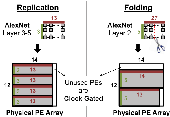
Fig. 32. Mapping uses replication and folding to maximized utilization of PE array [96].
