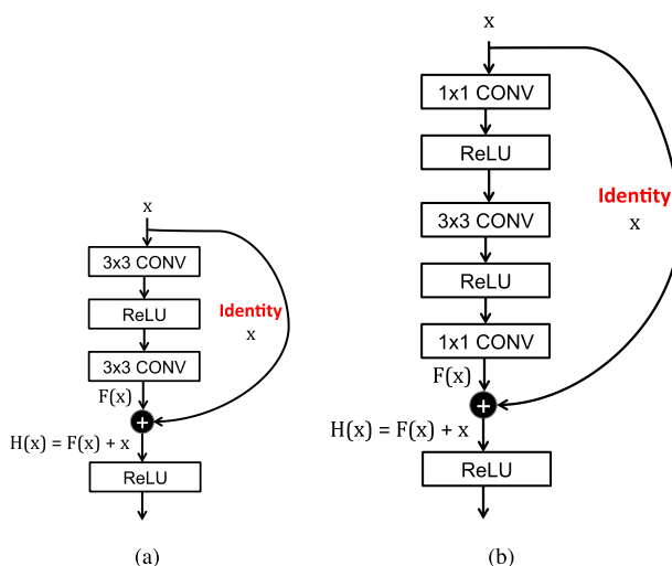
Fig. 15. Shortcut module from ResNet [15]. Note that ReLU following last CONV layer in short cut is after the addition. (a) Without bottleneck. (b) With bottleneck.
