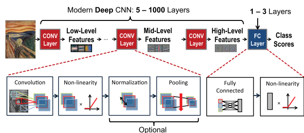
Fig. 10. Convolutional neural networks.
