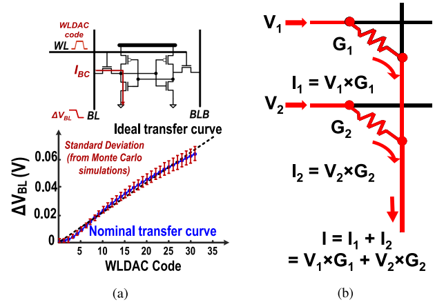
Fig. 36. Analog computation by (a) SRAM bit cell and (b) nonvolatile resistive memory. (a) Multiplication performed by bit-cell (Figure from [104]). (b) G_i is conductance of resistive memory (Figure from [106]).
