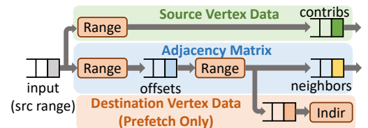
Fig. 5. DCL pipeline for Push PageRank.
