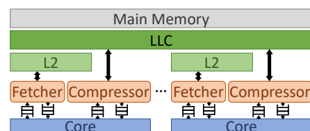
Fig. 9. SpZip architecture overview.
