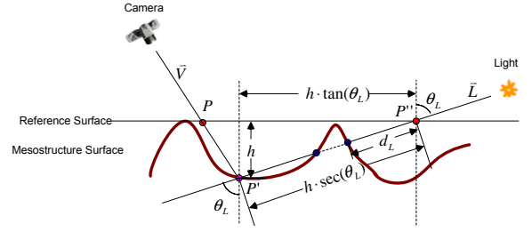
Figure 5: Shadow determination in VDM
