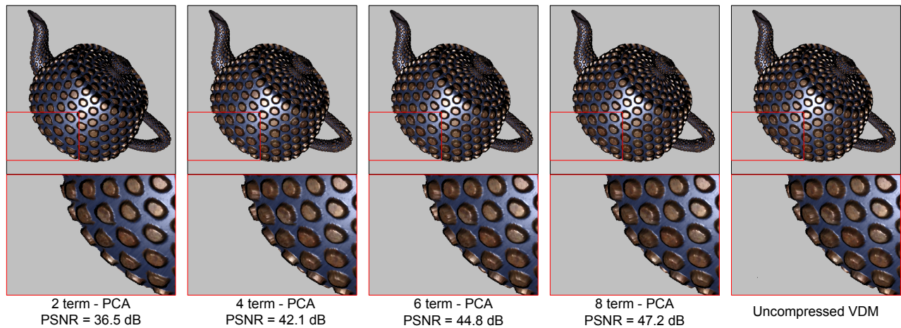
Figure 8: VDM rendering under different levels of compression.
