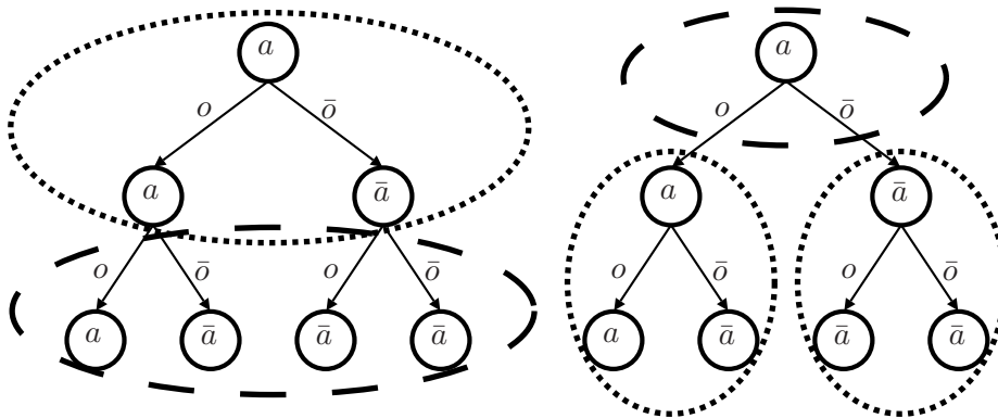
Figure 3: Difference between policy construction in MAA* (left) and dynamic programming (right) for an agent with actions a, \bar{a} and observations o, \bar{o} . The dashed components are newly generated, dotted components result from the previous iteration. MAA* ‘expands’ a partial policy from the leaves, while dynamic programming backs up a set of ‘sub-tree policies’ forming new ones.
