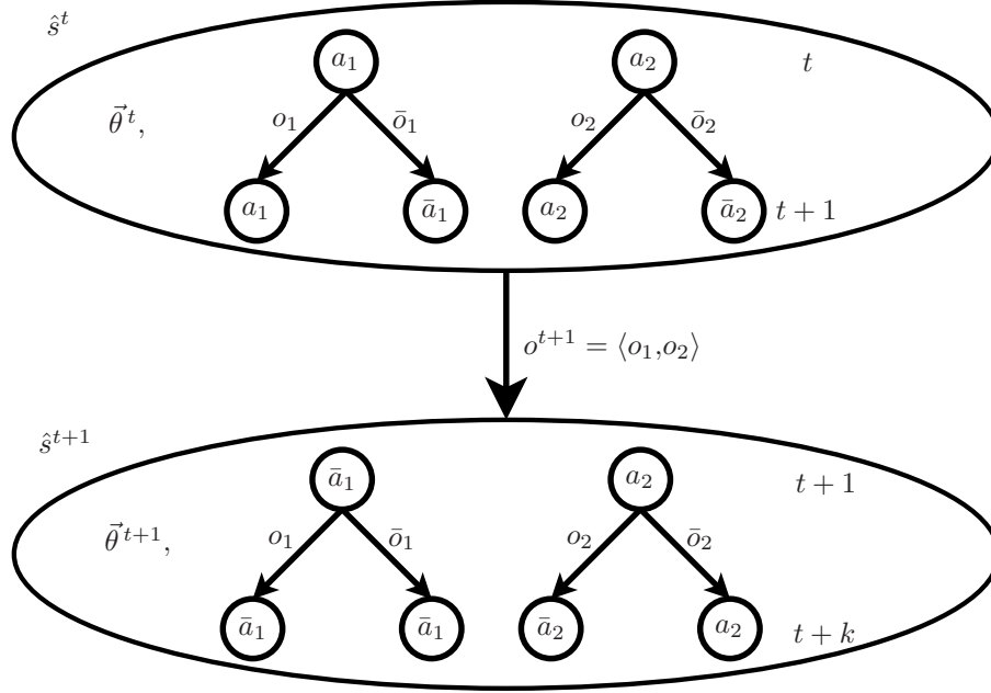
Figure 15: An illustration of the augmented MDP with k = 2 , showing a transition from \hat{s}^t to \hat{s}^{t+1} by action \hat{a} = \beta^t . In this example \vec{\theta}^{t-k+1} = (\vec{\theta}^{t-k+1}, \langle a_1, a_2 \rangle, \langle \bar{o}_1, \bar{o}_2 \rangle) . The actions specified for stage t are given by \beta^t(\langle \bar{o}_1, \bar{o}_2 \rangle) as depicted in Figure 14.
