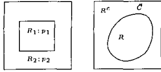
Fig. 1. Left Illustration of the foreground region ( R_1 ), the background region ( R_2 ), and the associated distributions ( p_1 and p_2 ). Right: Illustration of the curve ( \vec{C} ), the region inside the curve ( R ), and the region outside the curve ( R^c ).
