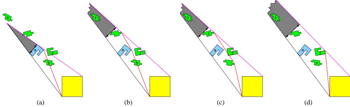
Figure 17: Growing the virtual occluders by intersecting objects with the active separating and supporting lines.
