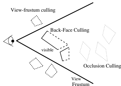
Figure 1: Three types of visibility culling techniques: (i) view frustum culling, (ii) back-face culling and (iii) occlusion culling.
