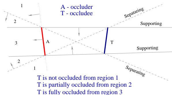
Figure 9: Supporting and separating planes.
