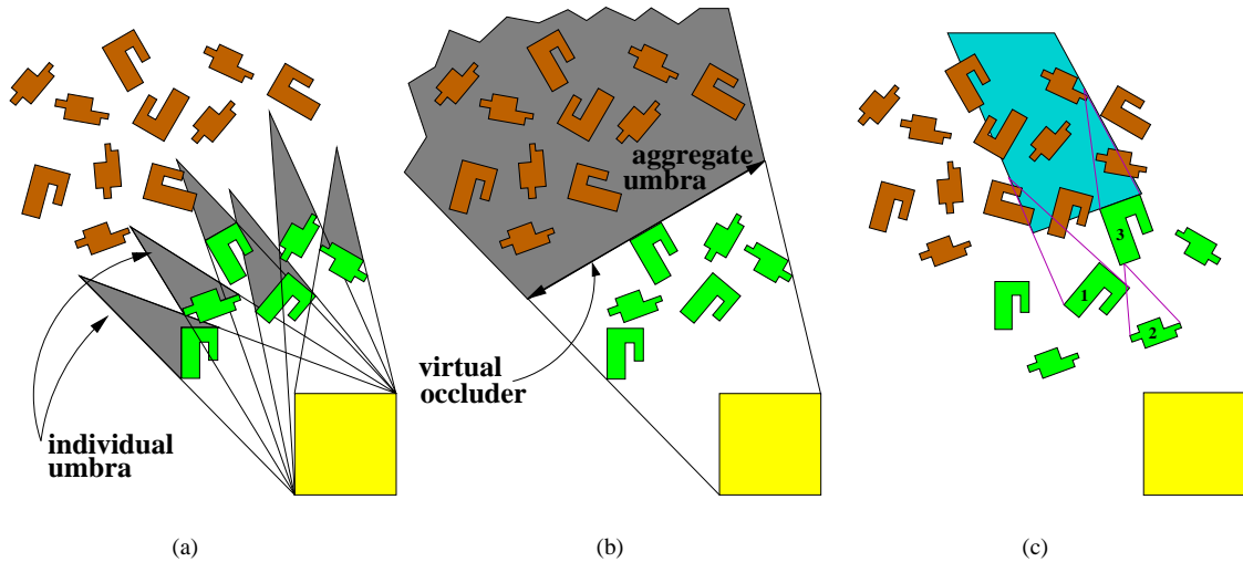
Figure 15: (a) The union of the umbrae of the individual objects is insignificant. (b) But their aggregate umbra is large and can be represented by a single virtual occluder. (c) The individual umbrae (with respect to the yellow view cell) of objects 1, 2 and 3 do not intersect, but yet their occlusion can be aggregated into a larger umbra.)
