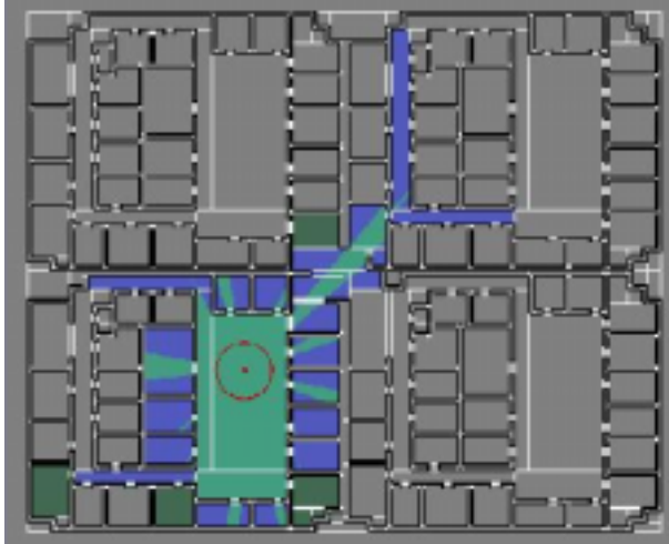
Figure 11: Results from [89] showing the potentially visible set from a given cell. Courtesy of Seth Teller, UC, Berkeley.
