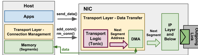
Figure 1: Tonic providing programmable transport logic in a hardware network stack on the NIC (sender-side).
