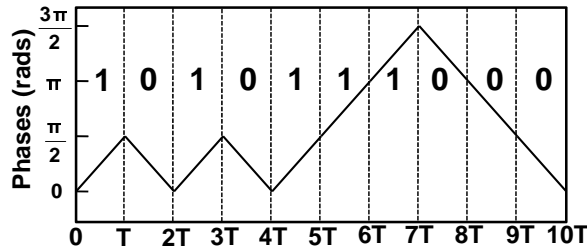
Figure 3 —Example MSK modulation. MSK represents a “1” bit of as a phase difference of \pi/2 over for an interval T . It represents a a “0” bit as a phase difference of -\pi/2 over T .
