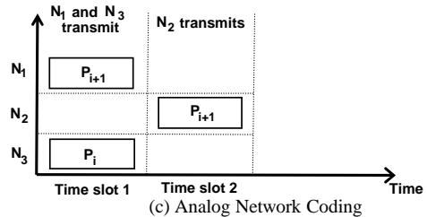
Figure 2—Chain Topology: Flows in one Direction. Nodes N_1 and N_3 can transmit at the same time. N_2 gets an interfered signal, but can recover N_1 's packet because it already knows the content of the interfering signal sent by N_3 . This reduces the time slots to deliver a packet from 3 to 2, producing a throughput gain of 3/2 = 1.5 .
