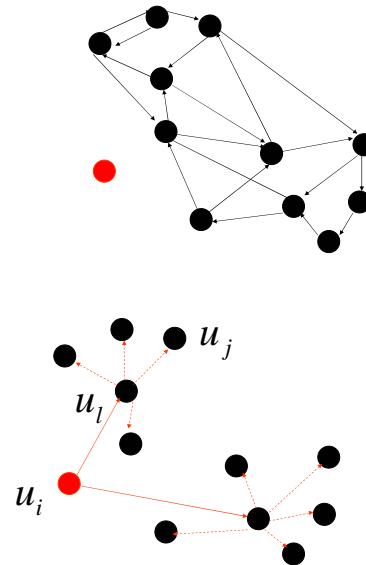
An overlay node applying Best Response wiring policy to the residual overlay graph
