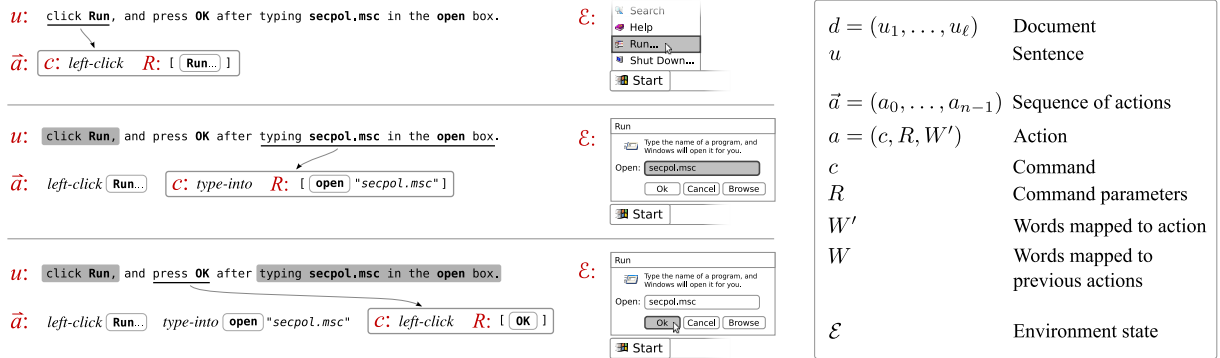
Figure 2: A three-step mapping from an instruction sentence to a sequence of actions in Windows 2000. For each step, the figure shows the words selected by the action, along with the corresponding system command and its parameters. The words of W' are underlined, and the words of W are highlighted in grey.
