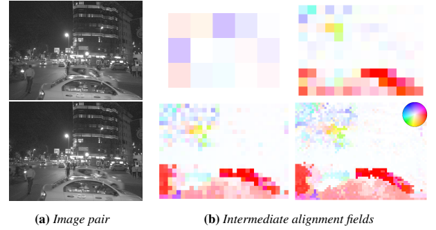
Figure 5: (a) A pair of 3 Mpix grayscale images. (b) The intermediate and final outputs of our multi-scale alignment, where hue and saturation indicate direction and magnitude of displacement (see the inset color circle). At the finest pyramid level (bottom right), tiles are 32 \times 32 pixels and the maximum displacement is 64 pixels. The large regions of saturated colors show that a hierarchical algorithm is essential; our method supports displacements up to 169 pixels. Although our displacements contain errors, they are cheap to compute and sufficiently accurate to use as input to our merging stage.
