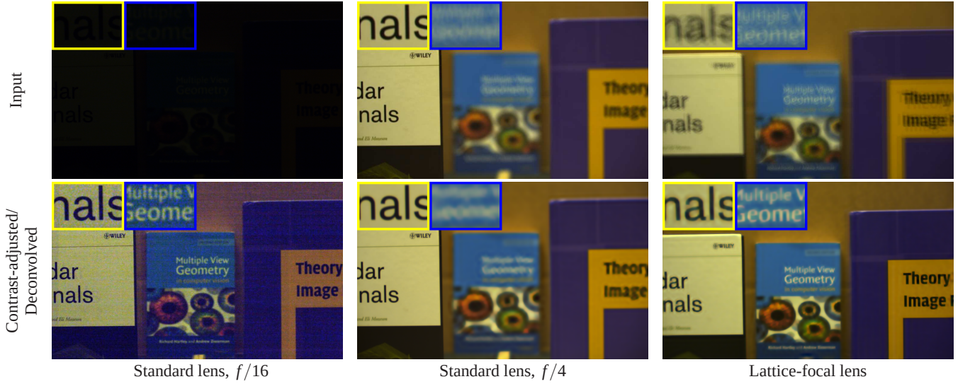
Figure 14: Comparison between a lattice-focal lens and a standard lens, both for a narrow aperture ( f/16 ) and for the same aperture size as our lattice-focal lens prototype ( f/4 ). All photos were captured with equal exposure time, so the f/16 image is very noisy. The standard f/4 image is focused at the white book, but elsewhere produces a defocused image. The lattice-focal output is sharper over the entire scene.
