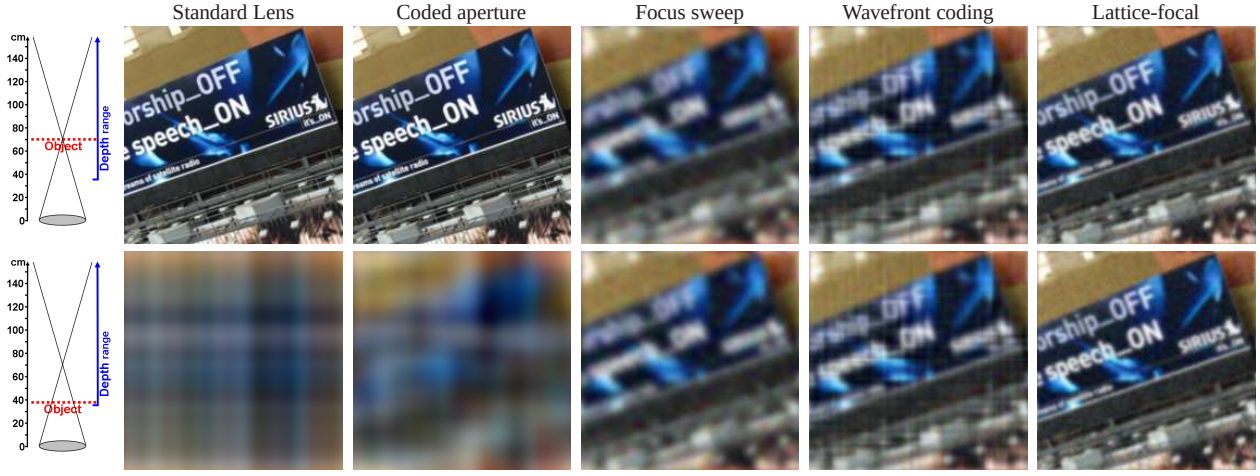
Figure 10: Synthetic comparison of image reconstruction at different object depths. Top row: object depth s = 0 , Bottom row: object depth s = -0.9 . Standard and coded lenses produce high quality reconstruction for an object at the focus depth, but a very poor one away from the focus depth. Focus sweep, wavefront coding and the lattice focal lens perform equally across depth. The highest quality reconstruction produced by our lattice-focal lens.
