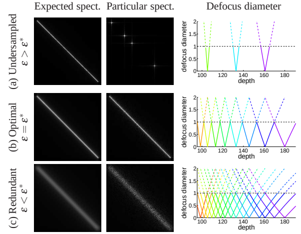
Figure 9: The lattice-focal lens with varying window sizes. Left: \omega_{x_0, y_0} -slice at \omega_x = 0.9\Omega, \omega_y = -0.9\Omega , through the expected spectrum. Middle: \omega_{x_0, y_0} -slice from a particular lattice-focal lens instance. Right: The defocus diameter over the depth of field. The expected spectrum improves when the windows number is reduced, but every particular lattice-focal lens becomes undersampled and does not cover the full depth range.
