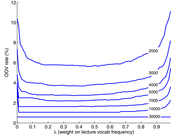
Fig. 1. OOV rate vs. \lambda weighting parameter for combining vocabularies obtained from the non-CS lectures and the CS course textbook. Each curve plots the OOV rate for a vocabulary constructed using the top N words from the combined set. The lecture and textbook frequencies are weighted by \lambda and (1 - \lambda) , respectively.
