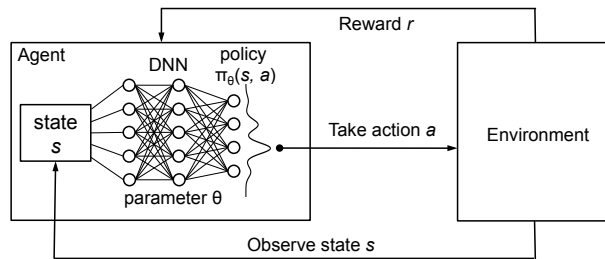
Figure 1: Reinforcement Learning with policy represented via DNN.
