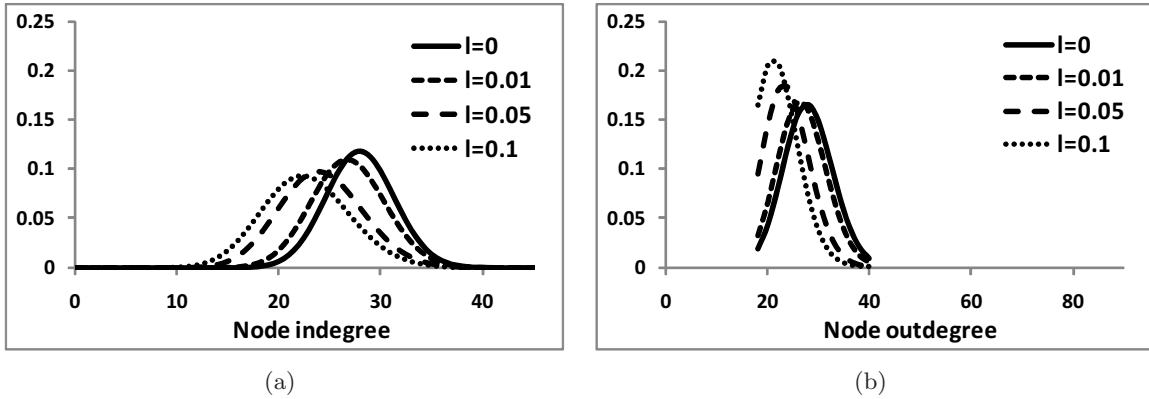
Figure 5: \mathcal{SEF} node degree distributions (exact, from Degree MC) for different loss rates \ell = 0, 0.01, 0.05, 0.1 ( d_L = 18 , s = 40 ).
