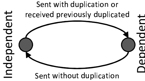
Figure 6: Dependence Markov Chain.
