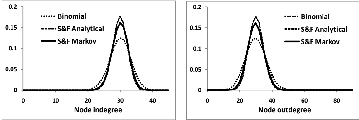
Figure 3: \mathcal{SEF} node degree distributions (analytical approximation and exact, from Degree MC) and binomial distributions with same expectation. s = 90 , d_L = 0 , \ell = 0 , ds(u) = 90 for each u .
