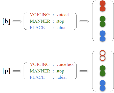
Figure 3: An illustration of IPA embeddings. Each phone is first represented by a vector of phonological features. The model first embeds each feature and then IPA embedding is obtained by concatenating all its relevant feature embeddings. For instance, the phone [b] can be represented as the concatenation of the voiced , stop and the labial embeddings.
