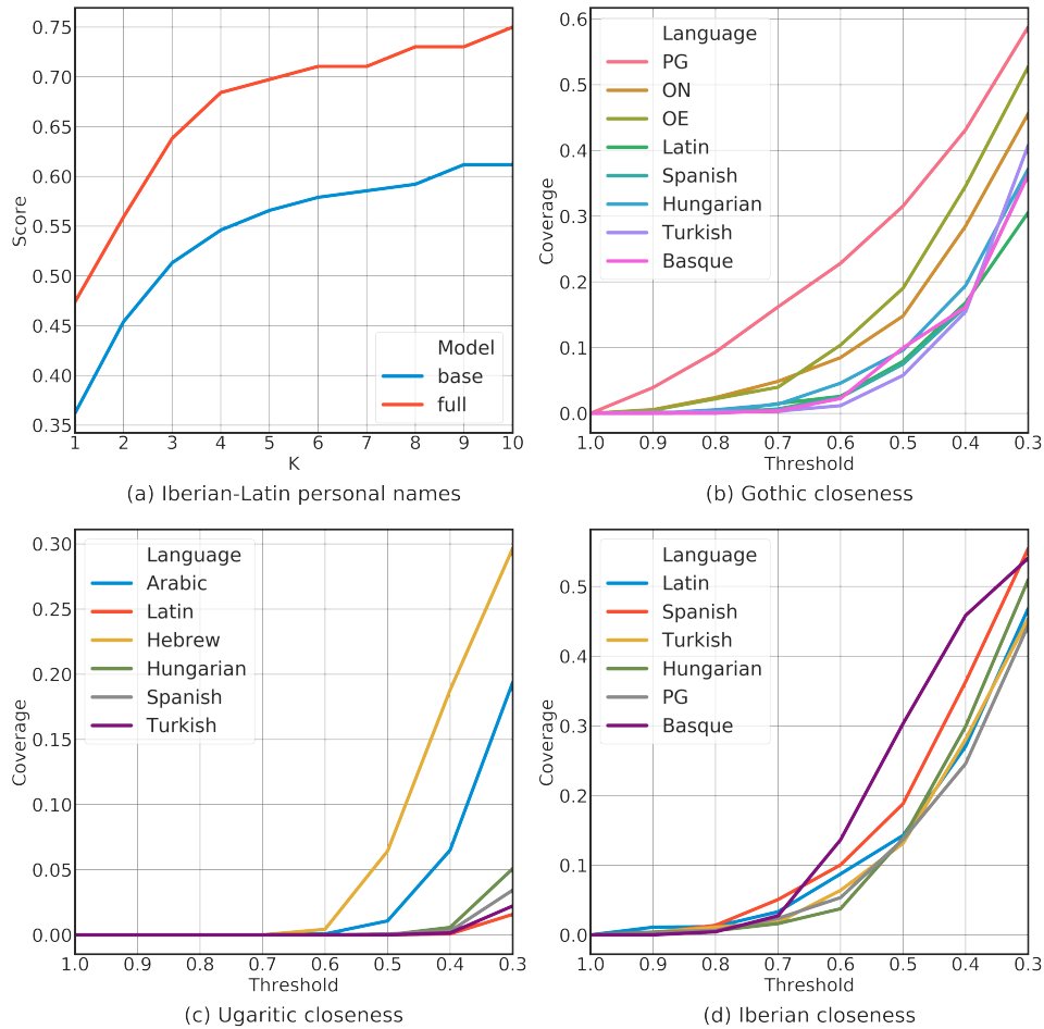
Figure 4: (a) P@K scores on Iberian using personal name recorded in Latin; (b), (c) and (d): Closeness plots for Gothic, Ugaritic and Iberian, respectively.
