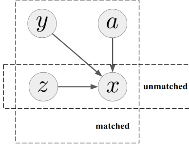
Figure 2: A graphical model representation for our framework to generate a span x . Characters in unmatched spans are generated in an i.i.d. fashion whereas matched spans are additionally conditioned on two latent variables: y representing a known cognate and a the character-level alignment between x and y .
