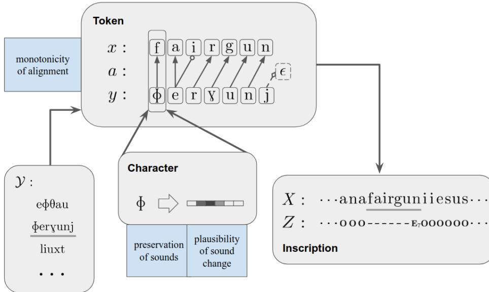
Figure 1: An overview of our framework which generates the lost texts from smaller units — from characters to tokens and from tokens to inscriptions. Character mappings are first performed on the phonetic alphabet of the known language. Based on these mappings, a token y in the known vocabulary \mathcal{Y} is converted into a token x in the lost language according to the latent alignment variable a . Lastly, all generated tokens, together with characters in unmatched spans, are concatenated to form a lost inscription. Blue boxes display the corresponding linguistic properties associated with each level of modeling.
