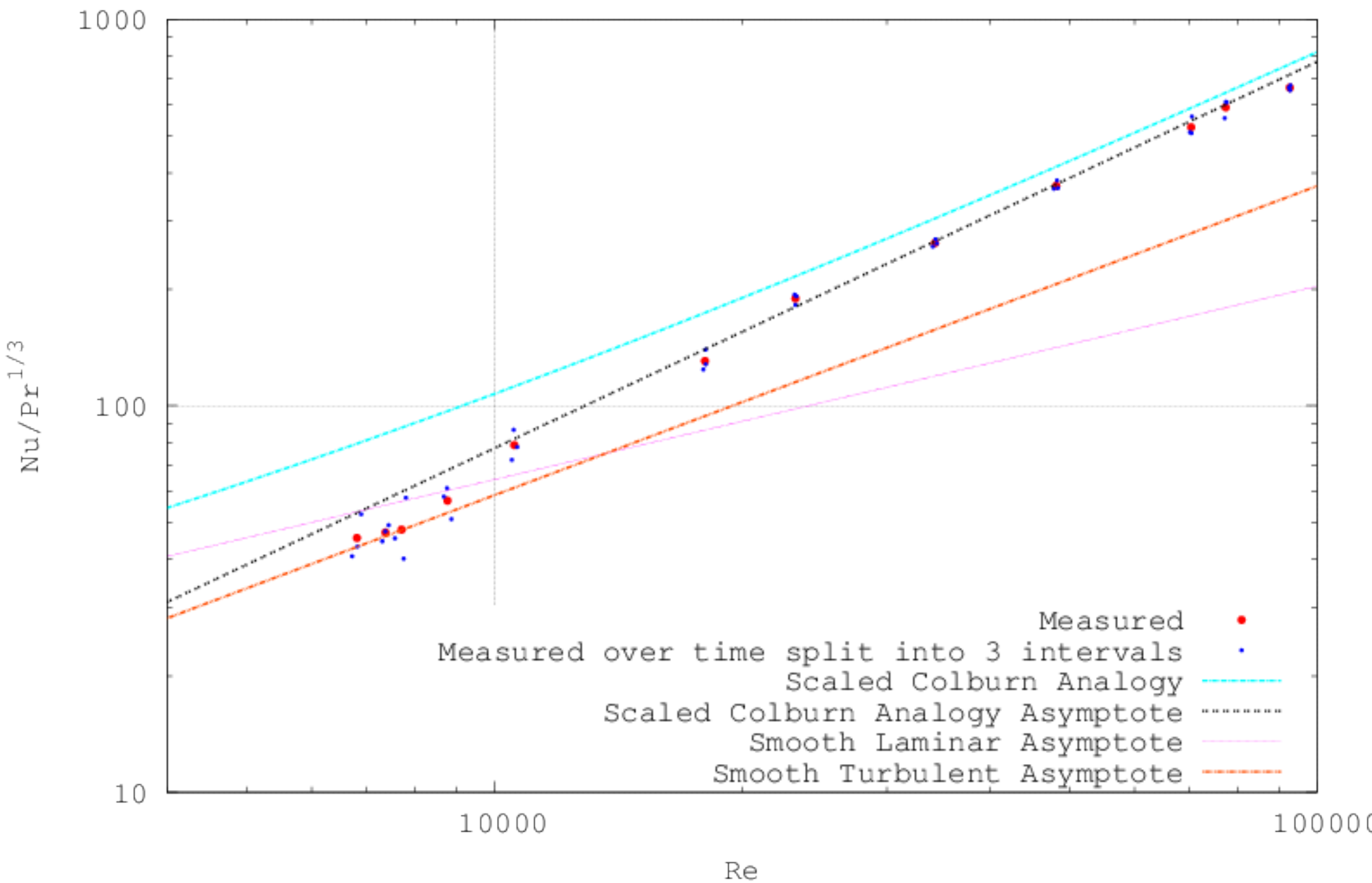
Measured versus Scaled Colburn Analogy
