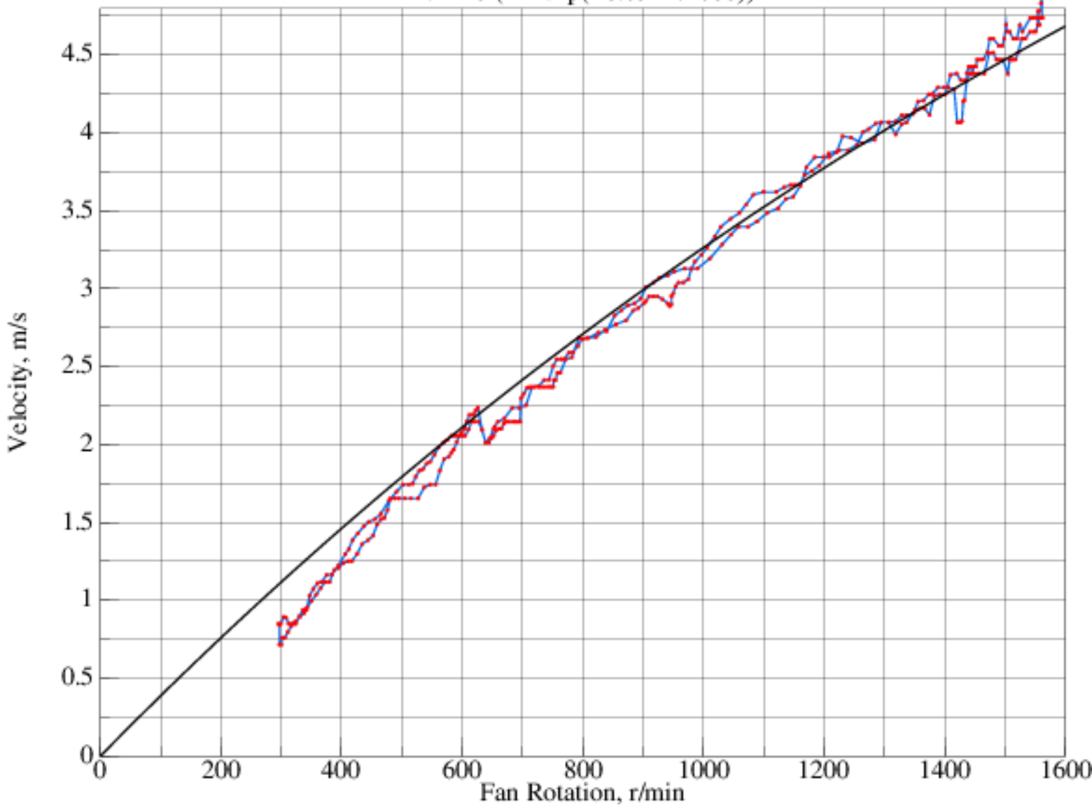
Airspeed vs Fan Rotation 20150802T193625Z, 21.68C, 54.2%, 100848P fit = 10 (1 - \exp(-0.632 r/1600))
