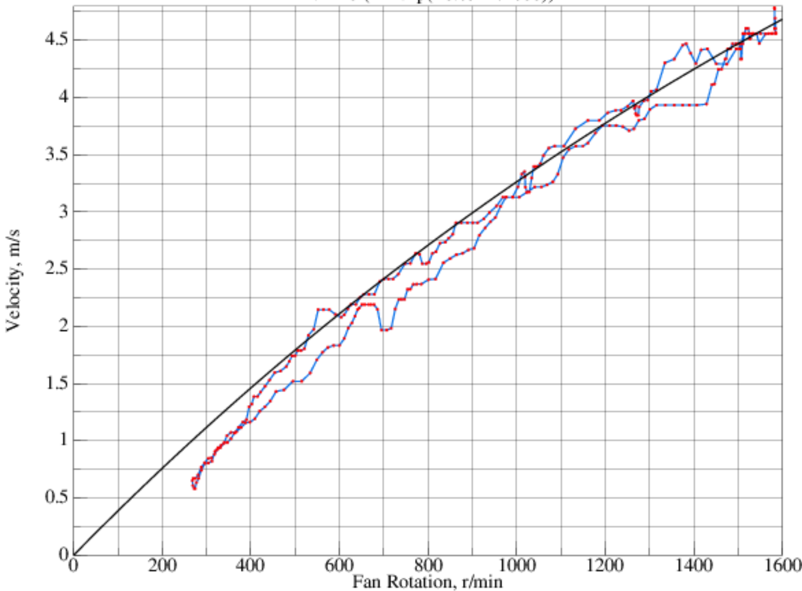
Airspeed vs Fan Rotation 20150802T195225Z, 22.19C, 53.0%, 100931P fit = 10 (1 - \exp(-0.632 r/1600))
