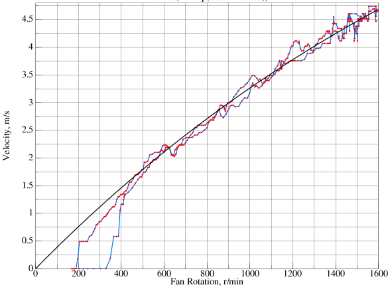
Airspeed vs Fan Rotation 20150729T023102Z, 21.19C, 54.6%, 101147P fit = 10 (1 - \exp(-0.632 r/1600))
