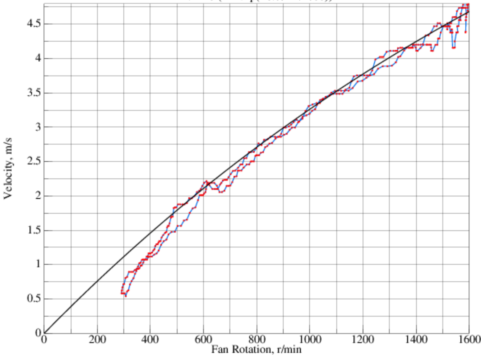
Airspeed vs Fan Rotation 20150731T214836Z, 20.96C, 54.3%, 100523P fit = 10 (1 - \exp(-0.632 r/1600))
