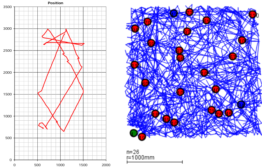
(a) The path from a single robot run- (b) The paths from many robots running ning BUMPREFLECT BUMPREFLECT
