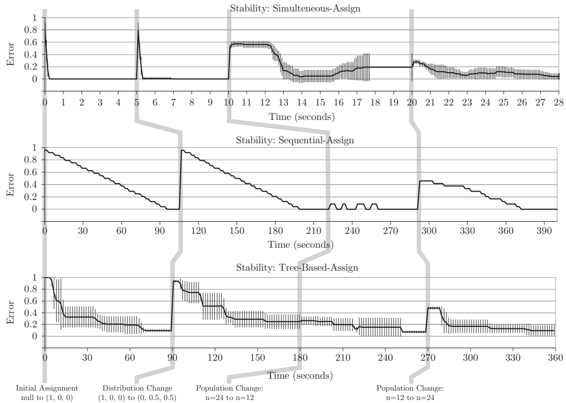
Figure 7-8: All of the algorithms are self-stabilizing when subject to external disturbances. This trio of graphs displays the recovery of the algorithms when subject to four different external disturbances; the initial convergence, a goal distribution change, removal of half of the robots, and replacement of the removed robots. Normalized error is plotted against time in all graphs, but the absolute times in each graph are different. Eight runs of SIMULTANEOUS-ASSIGNMENT produced the data on top. The algorithm performed well, but the data is partially corrupted by errors in our experimental setup. Some of this can be seen after t = 16 , as the error begins to rise, even though there is no disturbance (compare with Fig. 7-6). The plot of SEQUENTIAL-ASSIGNMENT shows the algorithm's steady progress. Multiple runs produced identical results, so only one example is shown here. The magnitude of the error after the first population change is small, but many robots needed to switch tasks, which can be very disruptive. The TREE-BASED-ASSIGNMENT algorithm was hindered by the same experimental setup as SIMULTANEOUS-ASSIGNMENT as well as the convergecast summation errors mentioned in the text. It converged accurately, but not rapidly.
