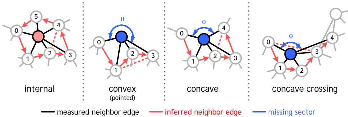
Figure 6-9: Illustration of the cyclic-shape algorithm’s progress when considering four boundary types, excluding the singleton case and local articulation points. The algorithm sorts the neighbors of a robot by their local bearing. It then starts at the first neighbor, and check for an inferred edge to the next neighbor. If a cycle through all the neighbors of a robot exists, then that is not a boundary. Note that in the concave crossing case, the robot is inside the interior of the polygon formed by the neighbor triangles, but is still classified a boundary.
