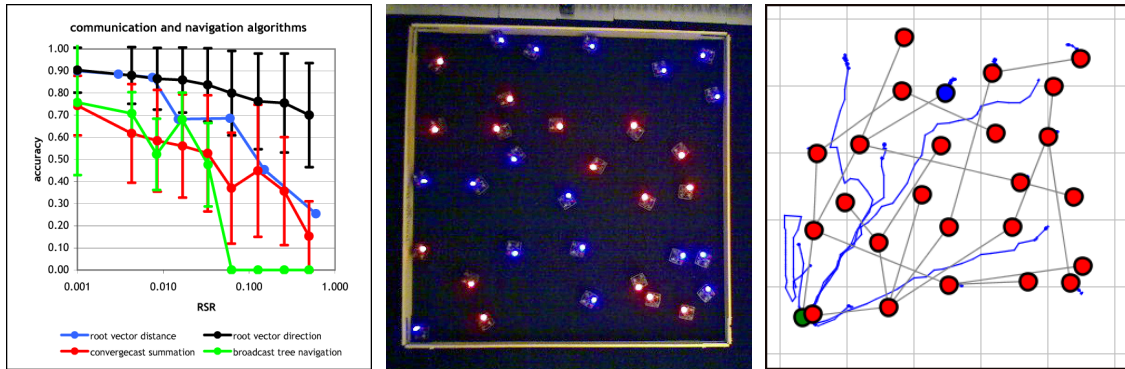
(a) Algorithm performance metrics (b) Robots performing broadcast (c) Experiment trace of broadcast tree construction from root at lower tree navigation left
