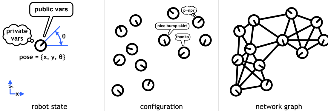
Figure 3-2: The robot state is the tuple of its global pose measured in an external reference frame and private and public variables, state_a = \langle ID_a, pose_a, privateVars_a, publicVars_a \rangle . A configuration is a group of robots. The configuration is valid if the network graph induced by connecting all robots whose separation distance, d < r , is connected.
