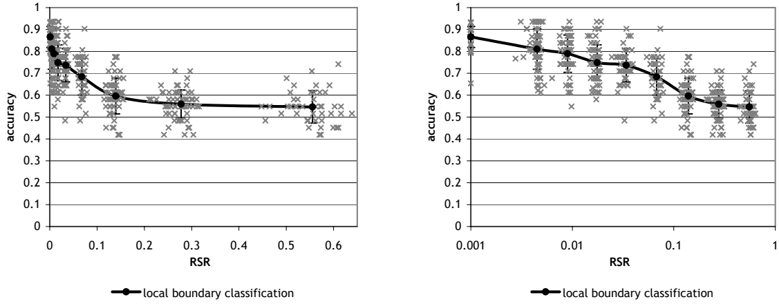
Figure 6-12: Accuracy of local boundary classification algorithm. Average accuracy in static configurations is 0.86. This drops as RSR increases, approaching 0.5, which is the ratio of perimeter to surface area in the 8' \times 8' workspace. The largest RSR tested occurs when the robots are moving at 80mm/s and communicating every 8 seconds, or 0.64 meters per communication round. This slow update allows them to sense their configuration in one location, but change their state when they are in another. (The same data is shown on both plots. left: linear x-axis, right: log x-axis).
