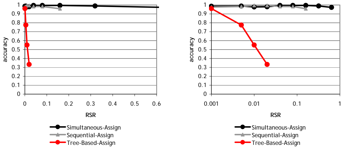
Figure 7-9: The accuracy of the three deterministic dynamic task assignment algorithms. The SEQUENTIAL-ASSIGNMENT and SIMULTANEOUS-ASSIGNMENT algorithms both essentially make a list of neighbors, and don't use communication for geometry or timely message delivery. Their performance is largely unaffected by the RSR. The TREE-BASED-ASSIGNMENT algorithm uses a broadcast = convergecast + rebroadcast communication structure, and its accuracy degrades sharply as RSR increases. The algorithm was not able to operate properly at RSRs greater than 0.02. (The same data is shown on both plots. left: linear x-axis, right: log x-axis)
