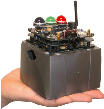
(a) A SwarmBot
