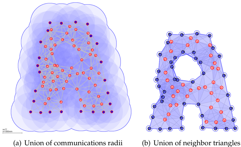
Figure 6-3: Illustrations of two possible boundary definitions. a: The boundary can be defined as: “robots whose communication disks contact the outer face.” However, when there are concavities in the configuration, this definition does not produce a contiguous boundary subgraph, as can be seen in the lack of boundary nodes in the concavity on the left hand side. Also, this definition does not detect the small void in this example. b: The global polygon formed from the union of all the triangles between a robot and each pair of its neighbors can be used to define the boundary. The shading indicates how many triangles are overlapping in a given area. Note the concavity on the left side of the configuration contains robots that are not on the exterior of the polygon. This definition would not include these robots, but they are needed to produce the contiguous boundary that is drawn in blue.
