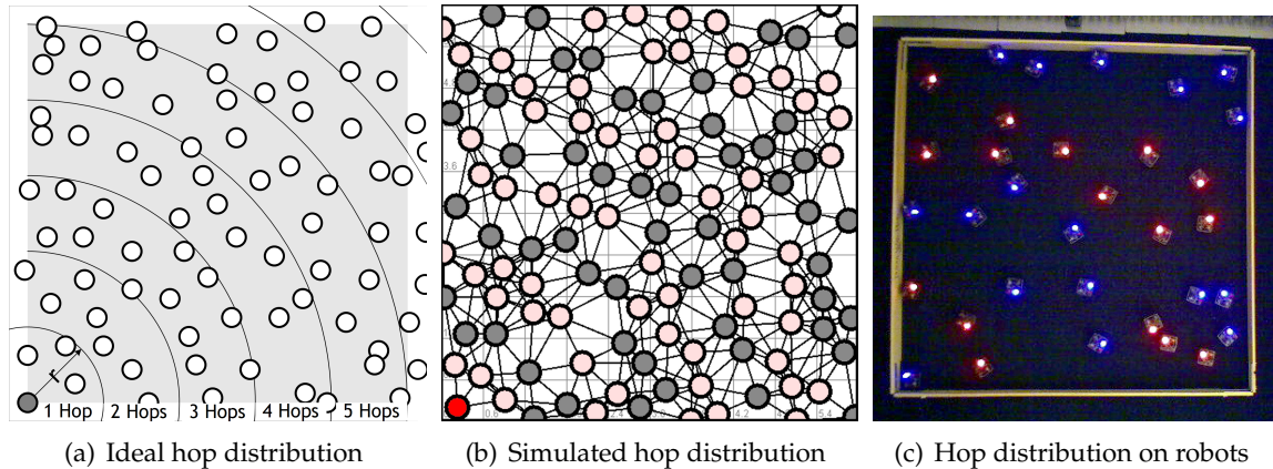
Figure 5-1: Broadcast tree construction. a. The ideal distribution of communication hops would be a series of concentric circles around the root. b. A simulation of a hops distribution from a root robot in the lower-left. Robots with an odd and even number of hops are drawn in light red and grey respectively. c. Picture of the robots indicating their hops from the root of a broadcast tree. The root is the single blue robot located in the lower left corner of the workspace. Robots that are located an even number of hops from the root are flashing their blue light, those located an odd number of hops are flashing their red light.
