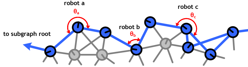
Figure 6-15: The turning angle is \theta_a - \pi , where \theta_a is the angle swept by the missing sector of robot a .
