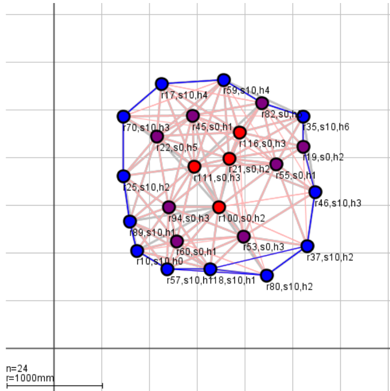
Figure 6-13: Boundary routing helpers add redundancy to the boundary subgraph, which can increase the stability considerably. This illustration is from a log file from an experimental run. Boundary subgraph routing helpers are drawn in purple, regular boundary robots in blue, and interior robots in red. Note that the helpers have patched a break in the boundary near the top of the configuration.
