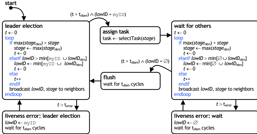
Figure 7-4: Sequential assignment algorithm finite-state machine diagram. The loop structures execute once each round.
