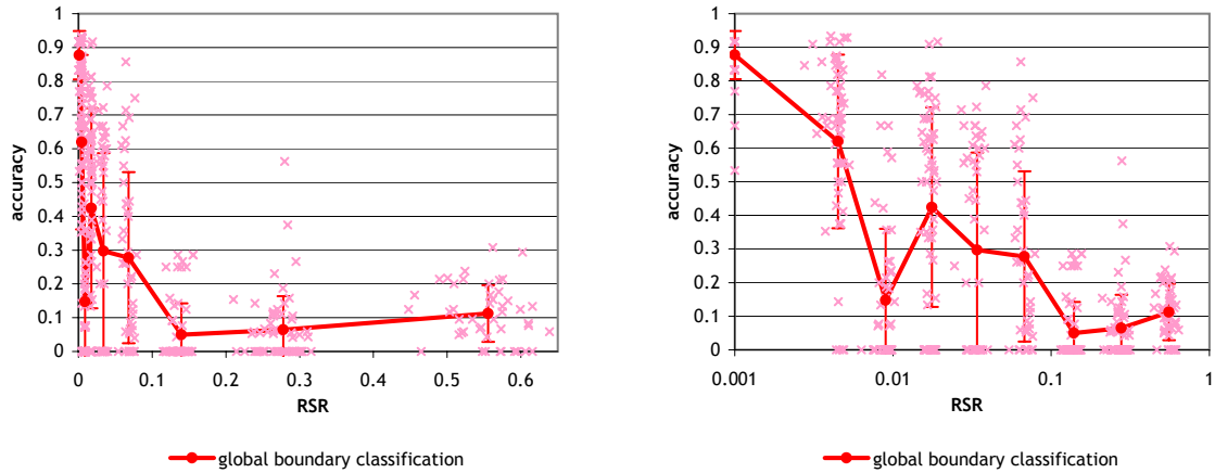
Figure 6-19: Accuracy of global boundary classification algorithm. (The same data is shown on both plots. left: linear x-axis, right: log x-axis).
