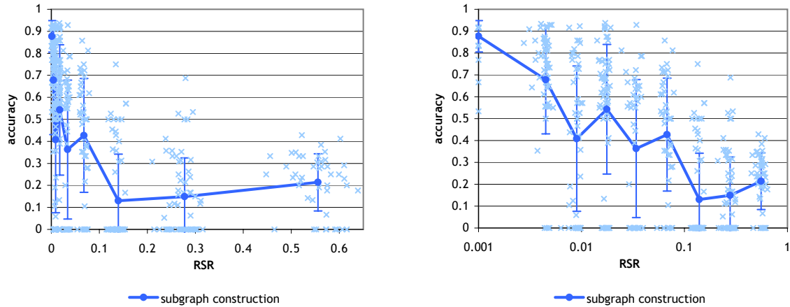
Figure 6-14: Accuracy of boundary subgraph construction algorithm. (The same data is shown on both plots. left: linear x-axis, right: log x-axis).
