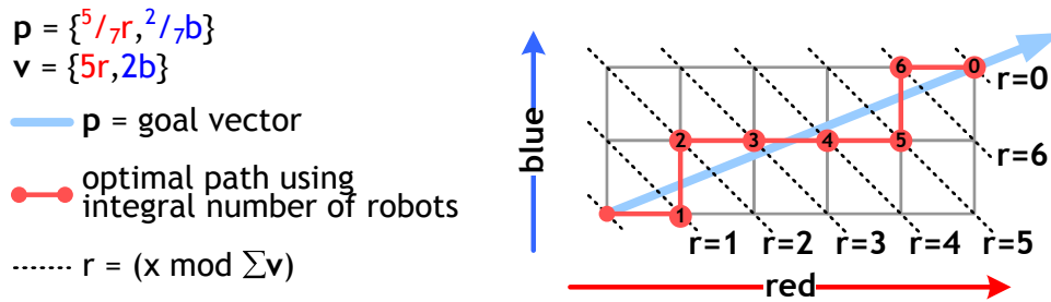
Figure 7-3: Illustration of the minimal representation from the sequential binning from Figure 7-2. The desired task assignment is again \mathbf{P}_{\text{goal}} = (\frac{5}{7}, \frac{2}{7}) .
