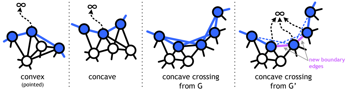
Figure 6-21: We want to show that each node on the external boundary has a path to infinity, but the concave crossing case causes trouble, as it is on the interior of the configuration polygon of the graph G . We construct a new graph, G' , with crossing edges removed and new edges defined as boundaries (purple edges). In the graph G' , each boundary node has a path to infinity.
