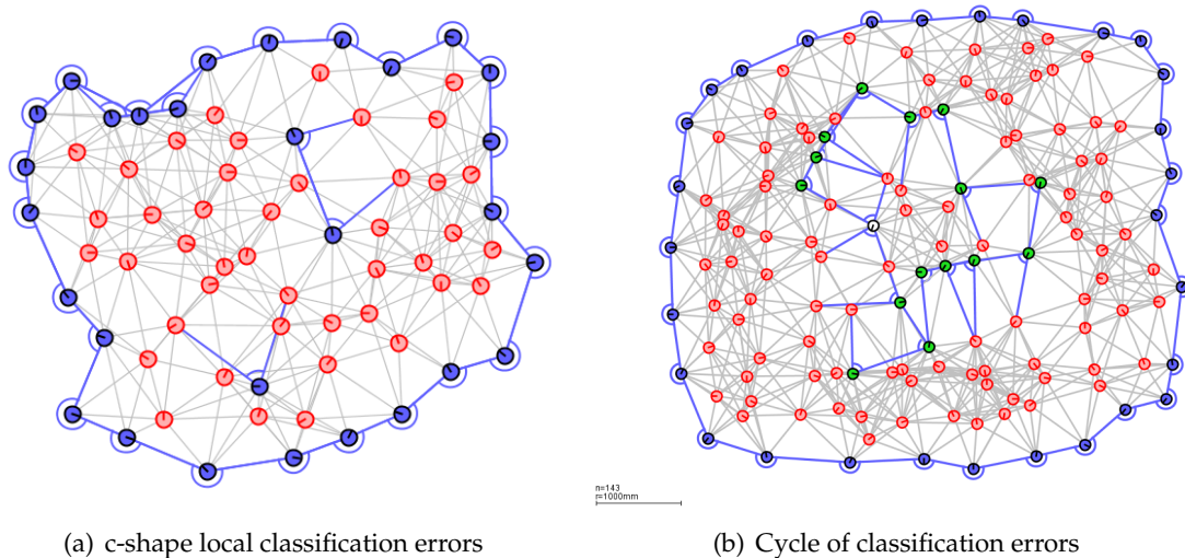
Figure 6-10: a. Because the c-shape algorithm only uses local network geometry, it is possible for robots that are on the interior of the network to be classified as boundaries. b. It is even possible to construct a cycle of erroneously classified boundary robots, making this kind of error more difficult to detect.
