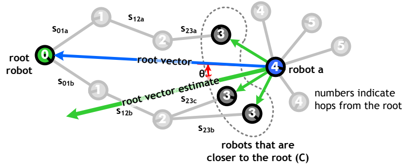
Figure 5-2: The broadcast tree can be used by any robot in the network to estimate the vector to the root. Robot a is four hops from the root. It has three neighbors that are closer than it is, one of them is its parent in the tree. Robot a can compute an estimate of the direction to the root by averaging the directions to its three neighbors that are closer to the root. The distance to the root can be estimated by summing the length of the edges the broadcast tree message has traveled to reach robot a .
