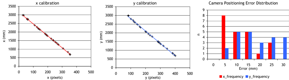
Figure 3-8: The calibration data and error histograms for the vision-based localization system. The x-axis shows measured error and the y-axis shows the bin population. The mean error over x and y axes is 15.4 mm. The system occasionally produces errors in excess of 30 mm, but refused to do so when we were testing it. These larger errors are very intermittent, occurring about once every 500 frames. These errors are very drastic shifts in position lasting for only one frame, and are easily filtered out.
