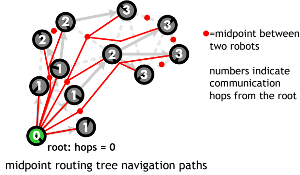
Figure 5-8: An illustration of a midpoint routing tree.
