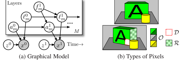
Figure 2: (a) Graphical model: x denotes a frame, \ell_m , a_m , and f_m are the support, appearance, and flow for layer m , and z controls the layer order. (b) An example of the three types of pixels that can occur in a new frame.
