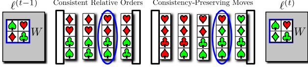
Figure 5: An example of the PGIMH proposals. A random window is chosen (left), W = \{\spadesuit, \clubsuit, \heartsuit, \diamondsuit\} , where suits indicate indices and colors indicate labels. A consistent relative order is selected at random. One of the N_W + 1 possible consistency-preserving moves is selected to produce \ell^{(t)} .
