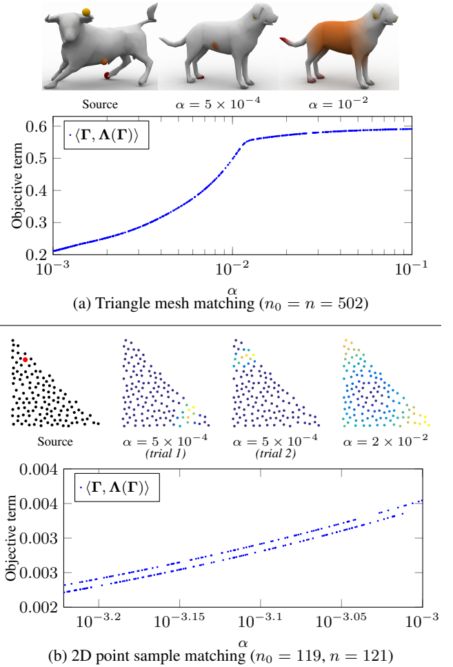
Figure 5: Sensitivity to initial guess of \Gamma for matching (a) surfaces and (b) planar point samples.
