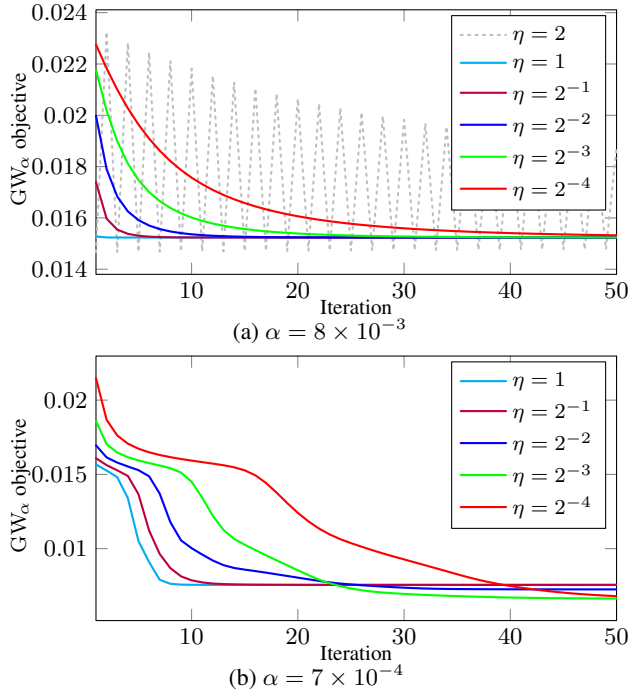
Figure 4: Convergence for the examples in Figure 2.
