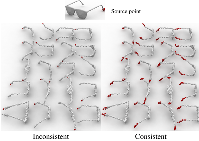
Figure 21: Consistent mapping via low-rank factorization reveals the left-right symmetric ambiguity of mapping between twenty models of eyeglasses ( \alpha = 10^{-3}, \beta = 1, n = 100 , rank 15).
