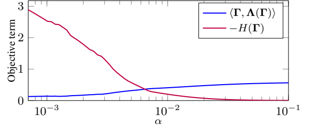
Figure 3: Dependence of objective terms on regularizer \alpha for the experiment in Figure 2.
