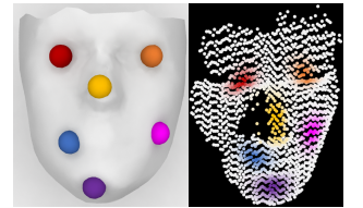
Figure 10: Point clouds.
