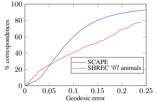
Figure 14: Benchmark tests from [Kim et al. 2011].
