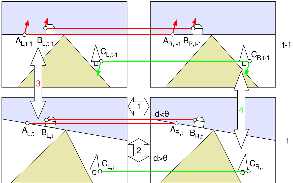
Figure 38: Our approach consists of four steps that are performed for each new frame: (1) Sparse stereo and putative matching. (2) Separate the sparse flow by disparity based on the threshold \theta that adapts to the vehicle speed. (3) Recover the rotational component of the camera motion from two distant points A_t and B_t using RANSAC to robustly deal with outliers. (4) Recover the translational component of the camera motion from one close point C_t again using RANSAC.
