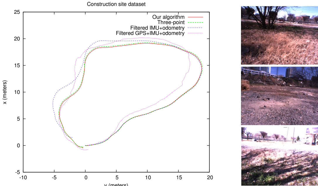
(a) Trajectories based on multiple algorithms and sensors.
