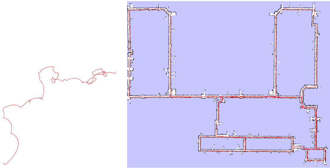
(a) Trajectory based on odometry.
