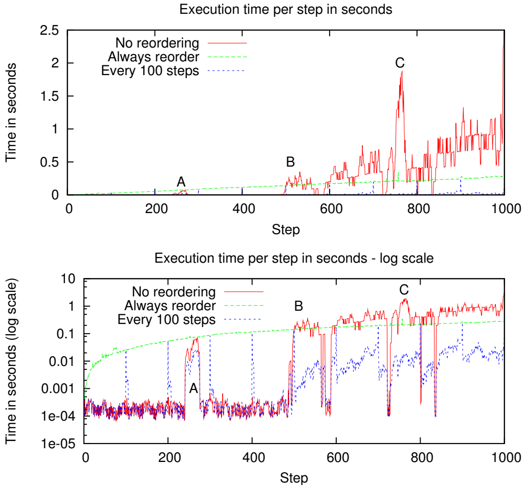
Figure 16: Comparison of execution times for the examples in Figure 15, shown in both linear (top) and log scale (bottom). Adding variables in the order that they appear in the estimation problem yields bad performance (continuous red) due to significant matrix fill-in as shown in Figure 15(b). Even reordering the variables after each step (dashed green) is sometimes less expensive. However, a considerable increase in efficiency is achieved by using fast incremental updates interleaved with only occasional variable reordering (dotted blue), here performed every 100 steps. Note especially that in the linear time figure this curve is near zero except for spikes caused by the periodic reordering.
