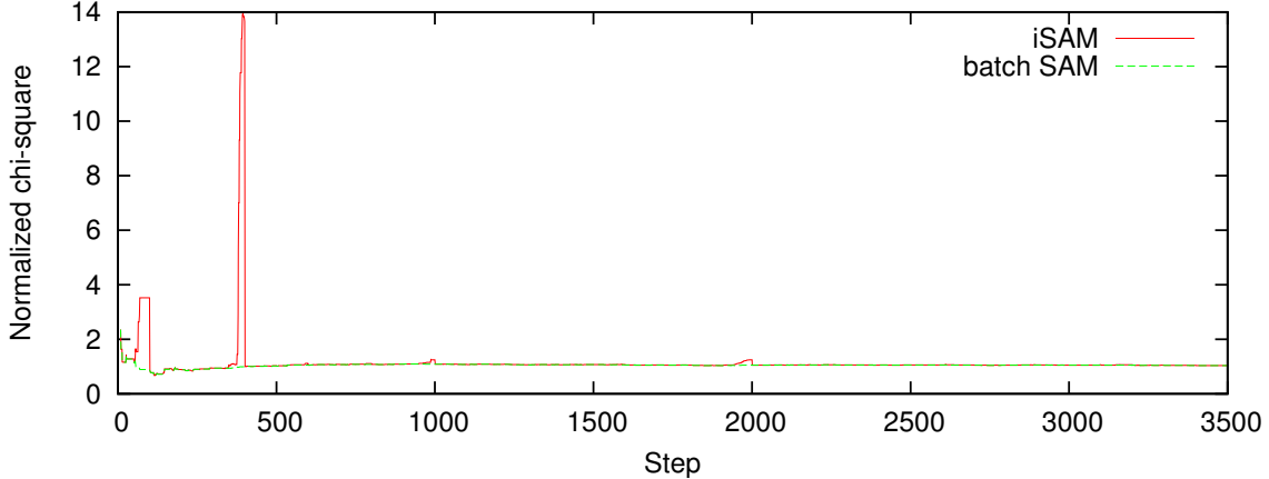
Figure 20: iSAM generally yields an exact solution, as shown by the normalized chi-square values for each iteration on the Manhattan world from Figure 19. I compare iSAM with a full nonlinear batch solution that iterates until convergence. The spikes are caused by temporary linearization errors after loop closing and always vanish during the periodic variable reordering step that also performs relinearization – see for example steps 400 and 1000.
