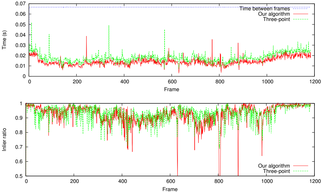
(c) Timing and inlier ratios comparing three-point with our algorithm.
