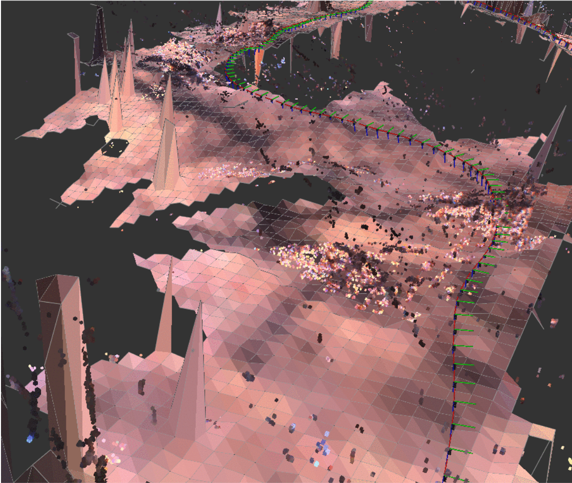
Figure 48: 3D ground surface reconstruction from dense stereo data, based on pose information from visual odometry. All pixels with available stereo information were used from frames selected at 3m intervals along the trajectory. A ground surface was fit by imposing a regular grid and taking the median of the height for each cell with a sufficient number of points. Only points not well described by the ground surface remain in the view. The result for this long sequence took only a few seconds to calculate.
