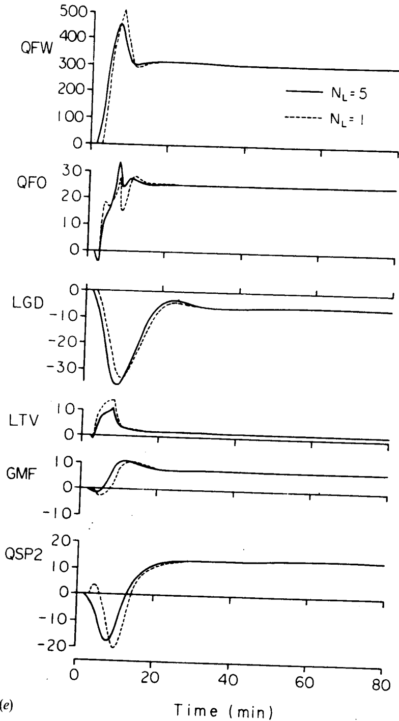
Figure 3. Closed-loop responses: (a) main steam pressure TP, (b) generator output MW, (c) controlled variables MST, TPL, RHT and NOX, (d) measurable outputs T1SH, TF, TECO and O2, (e) control variables QFW, QFO, LGD, LTV, GMF and QSP2.
