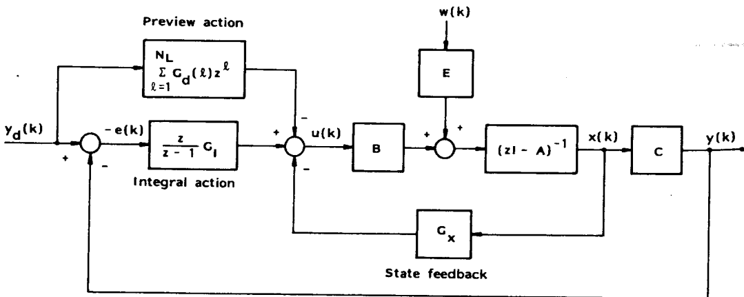
Figure 1. Overall configuration of feedback system.
