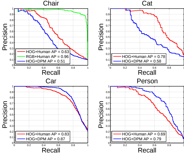
Figure 12: By instructing multiple human subjects to classify the visualizations, we show performance results with an ideal learning algorithm (i.e., humans) on the HOG feature space. Please see text for details.
