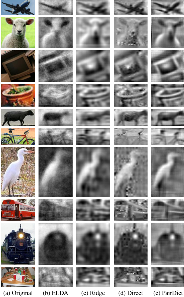
Figure 8: We show the results for all four of our inversion algorithms on held out image patches on similar dimensions common for object detection.
