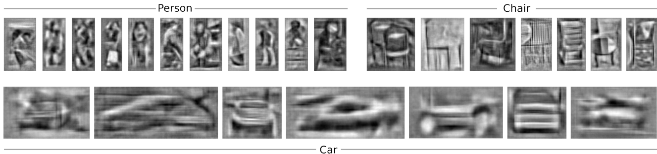
Figure 3: We visualize some high scoring detections from the deformable parts model [8] for person (top left), chair (top right), and car (bottom). Can you guess which are false alarms? Take a minute to study this figure, then see Figure 14 for the corresponding RGB patches.
