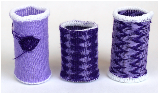
Fig. 14. Inside-out view of colorwork patterns: left, Intarsia patterns are created by modifying yarn paths; middle, plating uses two colors for every stitch creating a double sided pattern; right, Fair Isle patterns have a distinctive look on the reverse side due to “floating” yarns not used in stitches.
