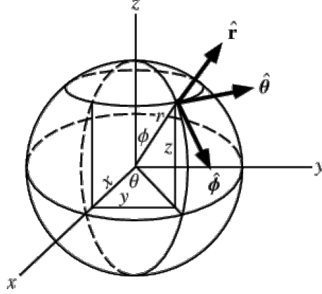
Figure 5.3: Zone Assignment in d dimensions. Because network coordinates have lower prediction error with d > 2 dimensions, it was important to generalize \hat{\theta} -routing with hyperspherical coordinates. With hyperspherical coordinates, each dimension “slices” the sectors of prior dimensions; thus, the total number of zones grows exponentially with the number of dimensions.
