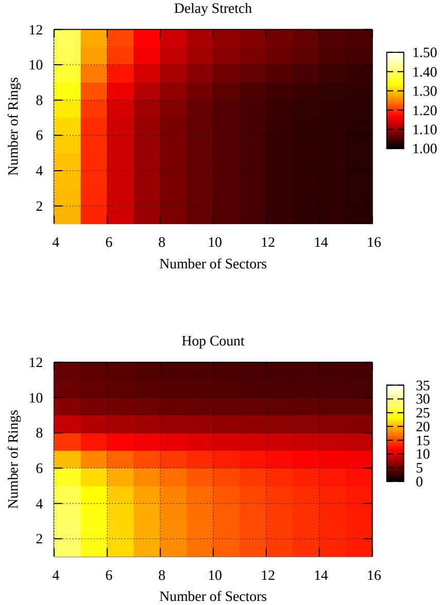
Figure 5.6: “Perfect” Routing Tables. For two-dimensional routing with “perfect” routing tables, far reaching rings and few angles result in queries that zig-zag across the coordinate space. Additionally, ring radii need to be tuned to the size and shape of the network to reduce hop count.
