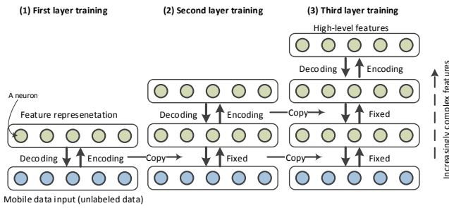
Fig. 2: Generative layer-wise training of a deep model. Each layer applies nonlinear transformation to its input vector and produces intrinsic features at its output.
