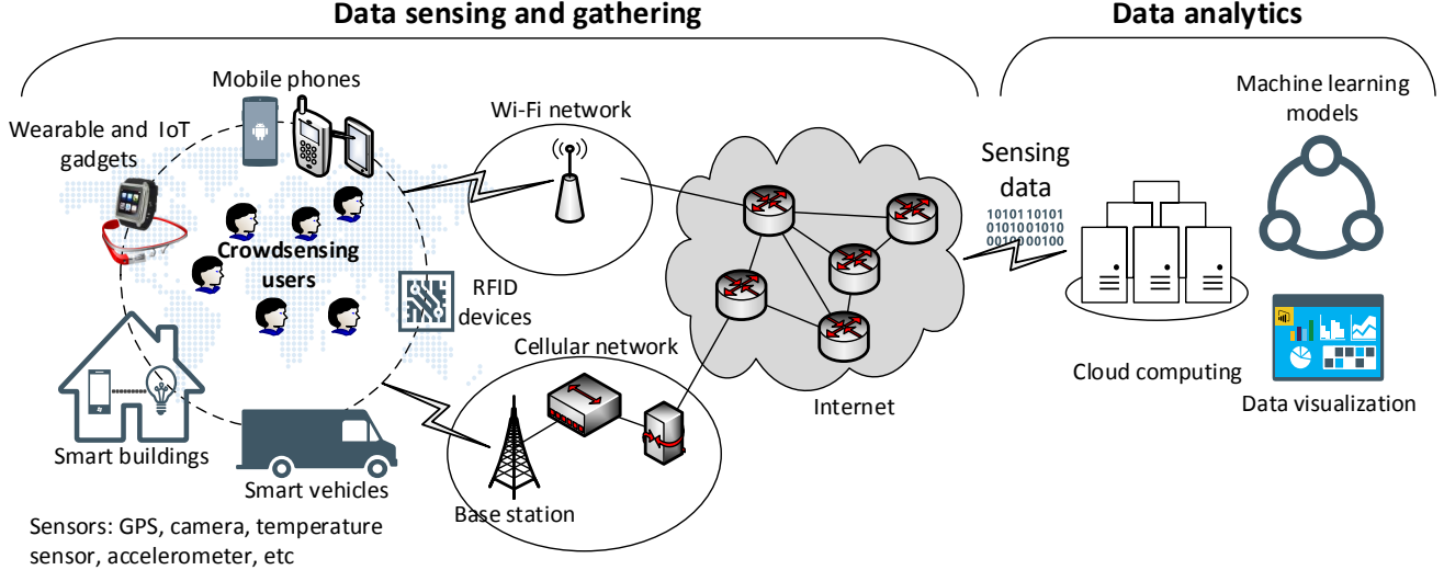
Fig. 1: System model of mobile crowdsensing.
