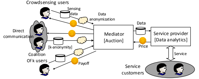
Fig. 3: System model of the privacy preserving crowdsensing framework supporting both data anonymization and identity generalization through crowdsensing coalition formulation. Cooperative users are connected using device-to-device (D2D) communication.
