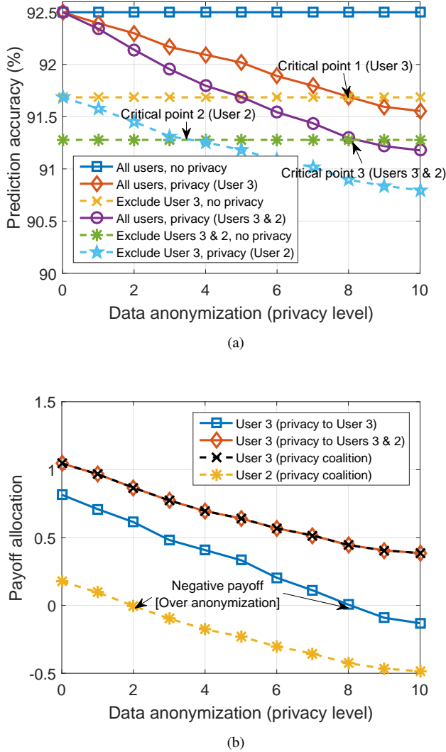
Fig. 5: Performance of the proposed privacy preserving framework under varied privacy levels. (a) The resulting accuracy of the deep learning service trained on the crowdsensing data. (b) The payoff allocation of Users 2 and 3. The privacy level is equal to the variance of the added Gaussian noise.
