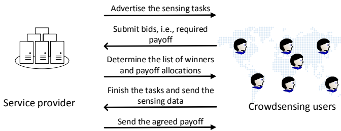
Fig. 2: Crowdsensing incentive mechanism as a reverse auction.
