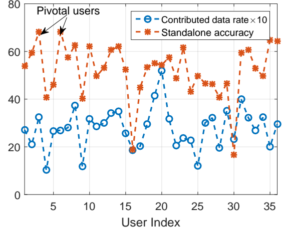
Fig. 4: User contribution to the crowdsensing service.
