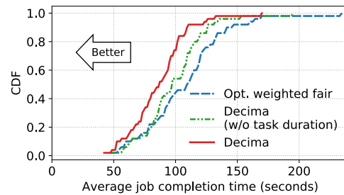
Figure 23: Decima performs worse on unseen jobs without task duration estimates, but still outperforms the best heuristic.
