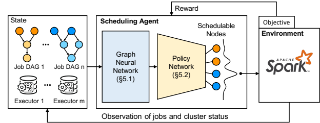
Figure 4: In Decima’s RL framework, a scheduling agent observes the cluster state to decide a scheduling action on the cluster environment , and receives a reward based on a high-level objective. The agent uses a graph neural network to turn job DAGs into vectors for the policy network , which outputs actions.
