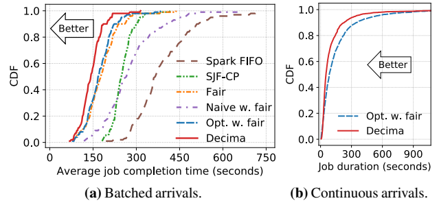
Figure 9: Decima’s learned scheduling policy achieves 21%–3.1× lower average job completion time than baseline algorithms for batch and continuous arrivals of TPC-H jobs in a real Spark cluster.
