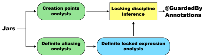
Figure 7: The structure of the abstract interpretation inference.
