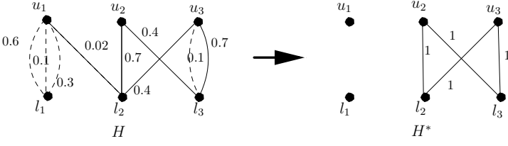
Figure 3: A solution with revenue 0.2
