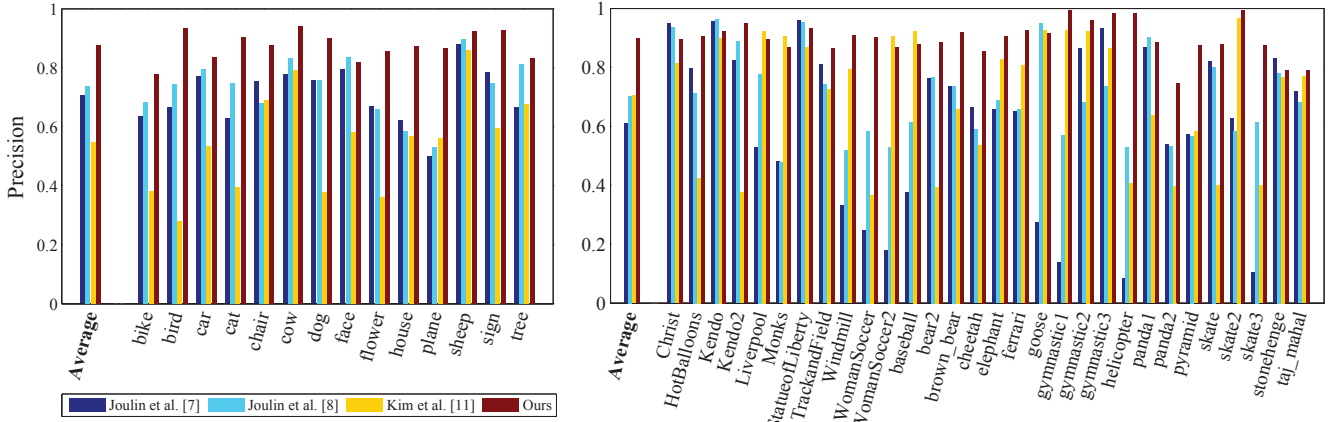
Figure 4. Segmentation accuracy on MSRC (left) and iCoseg (right) , measured as the ratio of correctly labeled pixels (both foreground and background), and compared to state-of-the-art co-segmentation methods (we performed a separate comparison with Object Cosegmentation [25]; see the text and Table 1). Each plot shows the average per-class precision on the left, followed by a breakdown of the precision for each class in the dataset.
