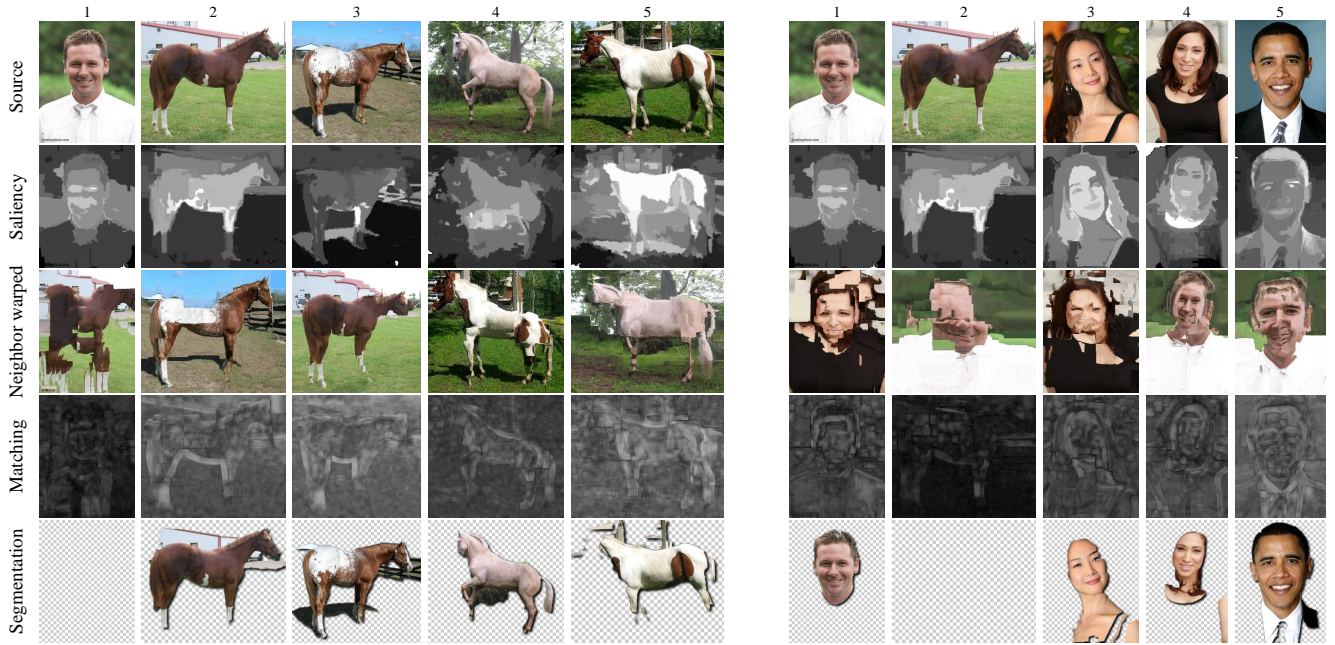
Figure 2. One of these things is not like the others. An illustration of joint object discovery and segmentation by our algorithm on two small datasets of five images each. The images are shown at the top row, with two images common to the two datasets – the face and horse images in columns 1 and 2, respectively. Left: when adding to the two common images three images containing horses (columns 3 – 5), our algorithm successfully identifies horse as the common object and face as “noise”, resulting in the horses being labeled as foreground and the face being labeled as background (bottom row). Right: when adding to the two common images three images containing faces, face is now recognized as common and horse as noise, and the algorithm labels the faces as foreground and the horse as background. For each dataset, the second row shows the saliency maps, colored from black (less salient) to white (more salient); the third row shows the correspondences between images, illustrated by warping the nearest neighbor image to the source image; and the fourth row shows the matching scores based on the correspondences, colored from black (worse matching) to white (better matching).
