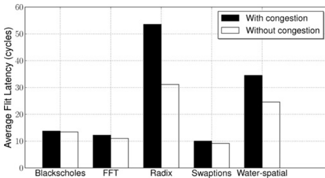
Fig. 12. Effect of congestion on flit latency for five SPLASH applications: for RADIX and WATER-SPATIAL, which both generate a lot of network traffic, not modeling congestion results in nearly 2 \times and 1.5 \times network latency underestimate; for BLACKSCHOLES, FFT and SWAPTIONS, which both have much less traffic, the difference, although present, is not significant. The results for the remaining SPLASH applications were similar: the congestion effect for high-traffic applications was similar to RADIX and for low-traffic applications resembled SWAPTIONS. (64-core system with 4 VCs, buffer depth is 4 flits).
