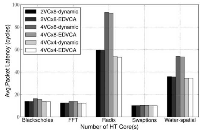
Fig. 13. In-network latency for different VC buffer configurations. Counter-intuitively, for heavy traffic loads like RADIX and WATER-SPATIAL, increasing the number of VCs from 2 to 4 while keeping the VC sizes constant at 8 flits actually increases in-network latency because packets can be buffered inside the network. When total VC memory size is held constant, doubling the number of VCs to 4 (and correspondingly halving their capacities to 4 flits) decreases latency as expected. For light traffic loads like the others, there are not so much congestion requirement for more virtual channels.
