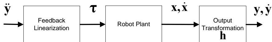
Fig. 8.5 – Feedback linearization and output transformation
