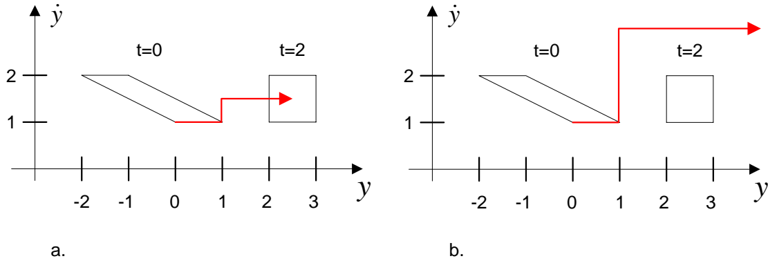
Fig. 5.14 – a. for a disturbance at t=1 with area 0.5, trajectory stays in tube; b. for a disturbance at t=1 with area 2, trajectory is pushed out of tube
