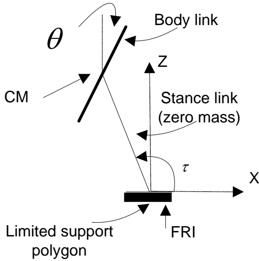
Fig. 3.8 – Simplified Model.
