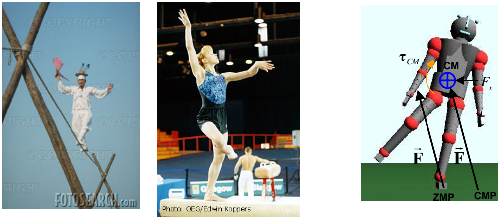
Fig. 1.19 – a. Tightrope and balance beam walking require rotational movement of the torso and non-contact limbs to maintain balance. b. Angular momentum about the CM allows the CMP to be moved beyond the limits of the support base.
