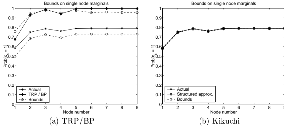
Figure 3. When to use a more structured approximation? (a) For strong attractive potentials, BP approximation is poor, as reflected by loose bounds on the actual marginal. (b) Kikuchi approximation [1] for same problem is excellent; corresponding bounds are tight.
