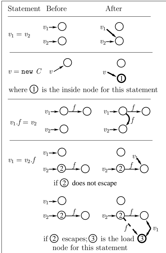
Figure 11: Graphical representation of intraprocedural transfer functions. Solid circles represent inside nodes, dashed circles represent load and parameter nodes, solid arrows represent inside edges, and dashed arrows represent outside edges. Bold circles and lines indicate potentially new nodes and edges.
