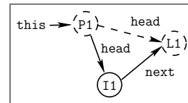
Figure 10: Points-to graph for Stack.push(int) .
