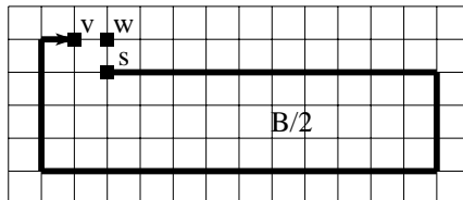
Figure 1. The learner reaches vertex v after B/2 steps in a depth-first search. Then it must interrupt its search and return to s . It cannot resume exploration at v to get to vertex w , because the known return path is longer than B/2 , the remaining number of steps allowed in this exploration phase. DFS fails.
