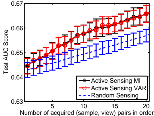
Figure 4: Experiments on NSCLC survival prediction. The features for the 2 views are listed in the left table, and the performance comparison of active sensing and random sensing is shown in the right figure. As baselines, training with full features (i.e., no sensing needed) yields 0.73; training with mean imputation (i.e., using the mean of each feature to fill in the missing entries) yields 0.62.
