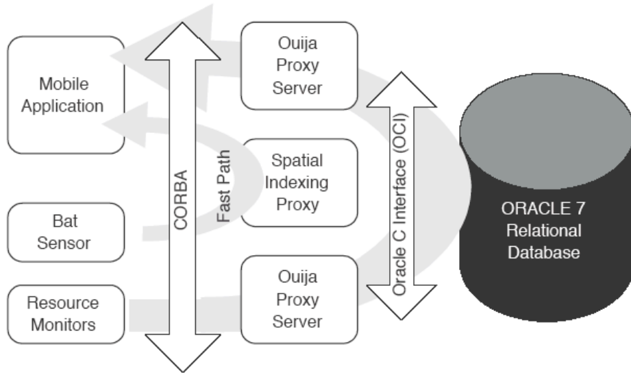
Figure 5. Three-tier architecture
